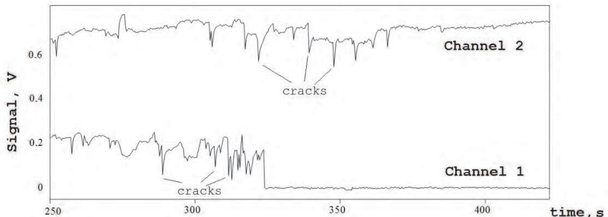
Fig. 8. Oscilloscope traces of photodetector signals in two channels of an adaptive fiber-optical measurement system which monitors crack the formation process in a solid state object
