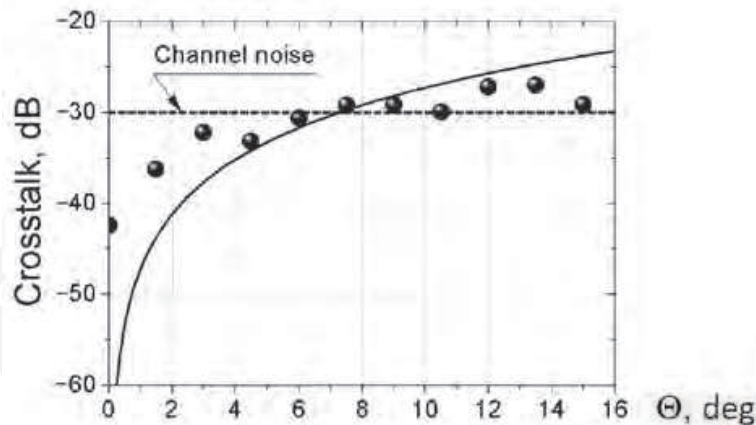
Fig. 13. Cross-talk between channels as function of angle between cross-hologram grating vector and normal to the crystal axis [001]: line represents theoretical dependency calculated in accordance with Eq.(14); markers are experimental data
