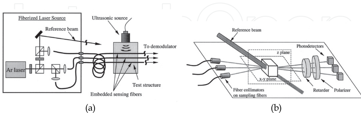
Fig. 9. Optical schematic of laser source and typical arrangement of sensing fibers (a) and three-channel adaptive demodulator based on angular multiplexing of dynamic holograms in BSO crystal (b)
