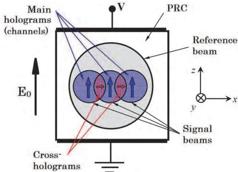
Fig. 10. Geometry of multi-wave mixing in PRC providing angular multiplexing of transmission dynamic holograms: all signal waves belong to horizontal plane ( xy ) and propagate in direction close to axis y ; the reference wave belongs to plane ( yz ) and makes the angle of 5^\circ with plane ( xy )
