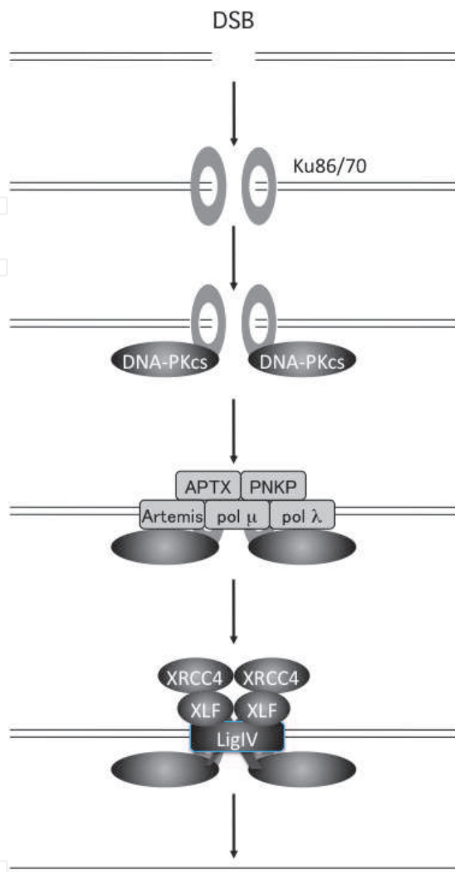
Fig. 1. Repair of DSB through NHEJ.
