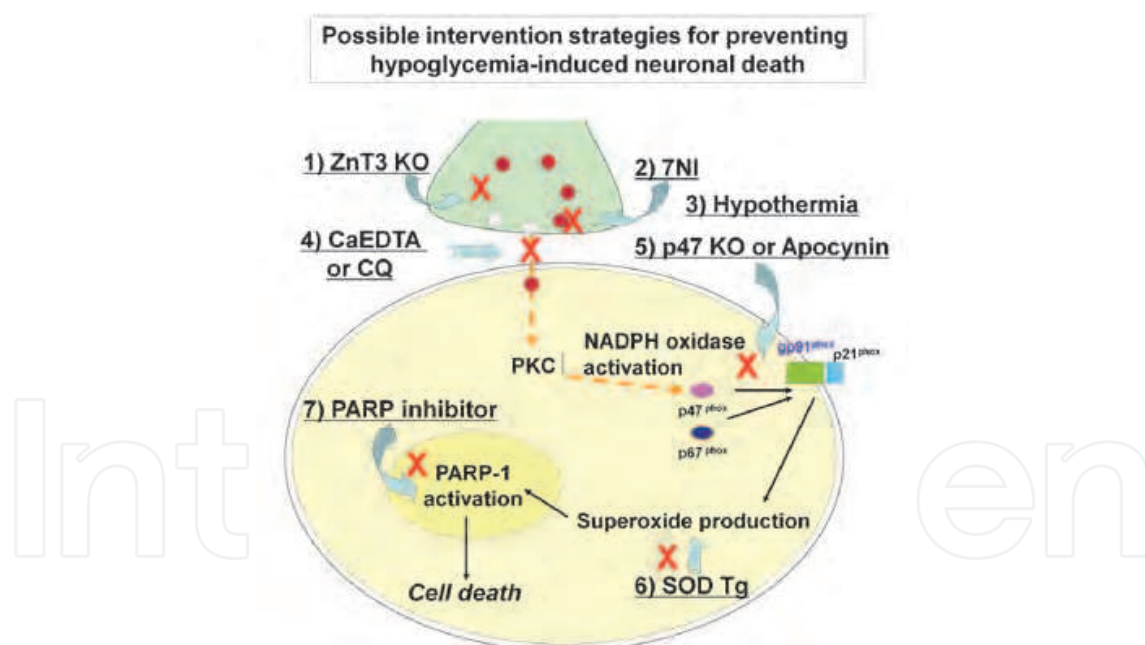
Fig. 9. Proposed intervention strategies for preventing hypoglycemia/ glucose reperfusion-induced neuron death. This schematic drawing indicates that hypoglycemia/ glucose reperfusion-induced neuron death can be prevented by several intervention methods. 1) Vesicular zinc content modulation by gene or chemical manipulation. 2) Vesicular zinc release inhibition by NO inhibitor. 3) Vesicular zinc release inhibition by hypothermia. 4) Zinc chelation in the extracellular space. 5) Inhibition of NADPH oxidase activation. 6) Scavenging or dismutating of reactive oxygen species. 7) Inhibition of PARP-1 activation. Round red colored dot represents ionic zinc. Symbol X represents intervention.
