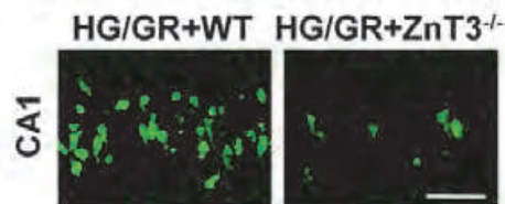
Fig. 5. Hypoglycemia/ glucose reperfusion-induced ROS production and neuronal injury is prevented by ZnT3 gene deletion in mice.
