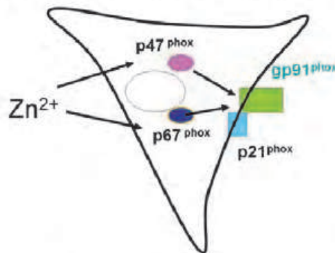
p47 and p67 translocation
