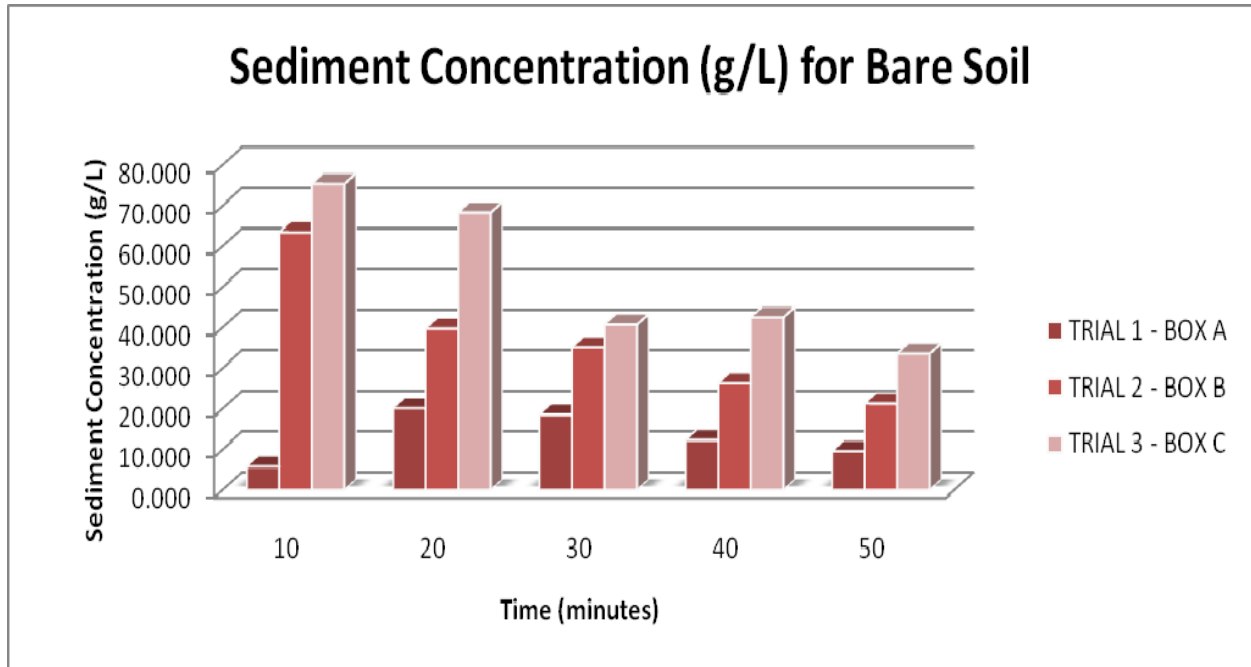
Fig. 7. Sediment Concentration (g/L) for Bare Soil
