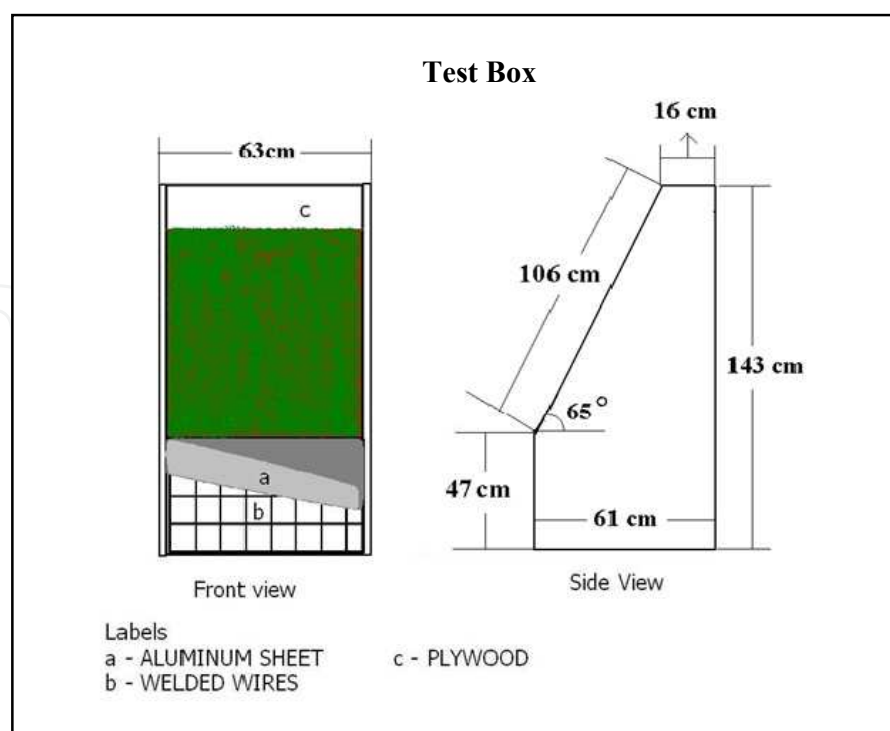
Fig. 1. Dimensions of the test box.
