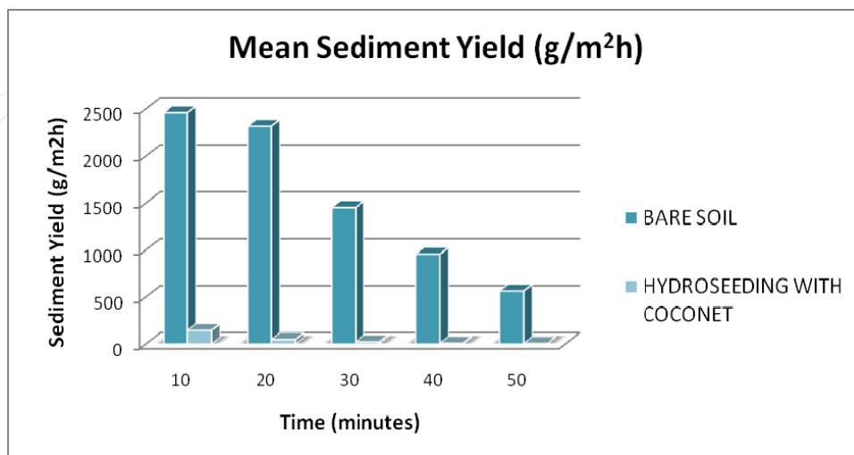
Fig. 12. Mean Sediment Yield of Bare Soil and Combination of Hydroseeding with Coconet Reinforcement
