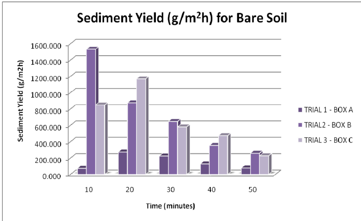
Fig. 10. Sediment Sediment Yield (g/m²h) for Hydroseeding with Coconet Reinforcement
