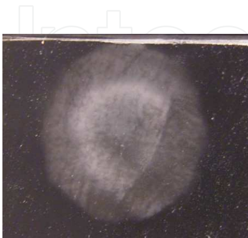
Fig. 9a. The photo of the track detector CR-39 covered by 11 mm Al filter. Detector CR-39 shows the tracks of protons with energies E_p > 0.8 MeV; \varphi_{1/2} \gg 14^\circ (cone half angle)
