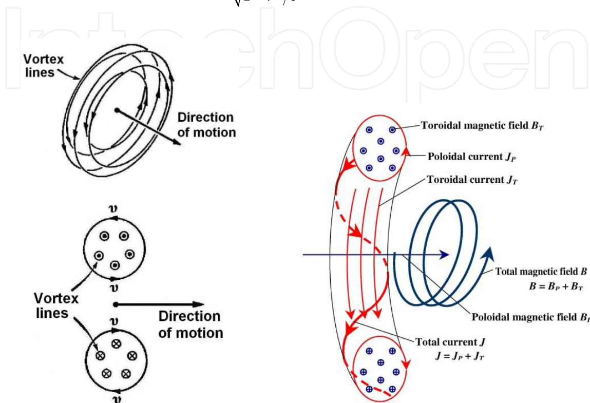
Fig. 8a. Vortex lines of moving potential vortex and its cross section
