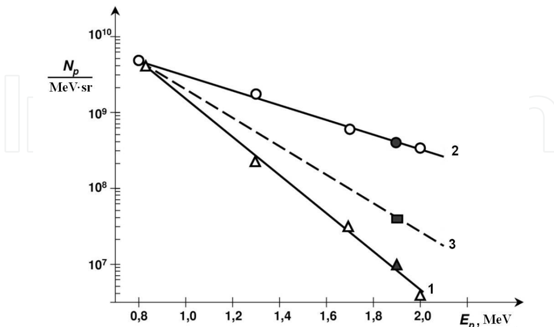
Fig. 5. Spectra of protons for various mechanisms of acceleration: (1) acceleration of protons from the front surface of the target toward a laser ray (Ti, 30 \mu\text{m} ; T \approx 180 keV); (2) acceleration of protons from the rear surface of the target in the outward direction (Ti, 30 \mu\text{m} ; T \approx 500 keV), and (3) acceleration of protons from the front surface of the target in the inward direction (LiF, 6 \mu\text{m} ; T \approx 250 keV). The open circles and triangles represent data from track detectors, while the closed circles, triangles, and boxes stand for data obtained on the basis of the activation procedure [ p(^7\text{Li}, ^7\text{Be})n , E_{thr} = 1.88 MeV].
