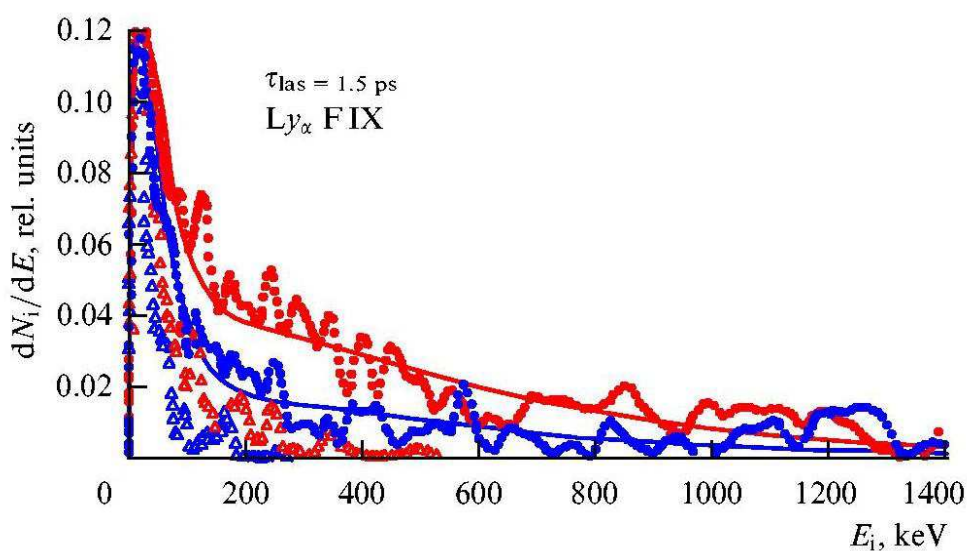
Fig. 7. Energy distribution of fast fluoride ions derived from the profile measurements of Ly \alpha line emitted by F IX ion. Top curve corresponds to ions moving towards the target, while bottom curve refers to ions moving outward from the target.
