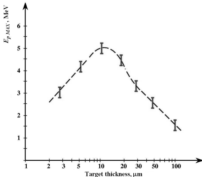
Fig. 6. Maximum proton energy E_{p\_MAX} as a function of the aluminum-foil thickness.
