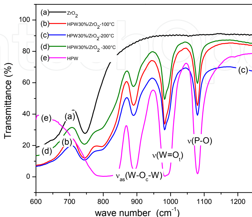
Fig. 3. FTIR spectra of \text{H}_3\text{PW}_{12}\text{O}_{40} (30% HPW) composites (a)- \text{ZrO}_2 ; (b)- \text{HPW}/\text{ZrO}_2 -100 °C (c) \text{HPW 30\%/ZrO}_2 -200°C; (d) \text{HPW 30\%/ZrO}_2 -300°C; (e)- HPW.
