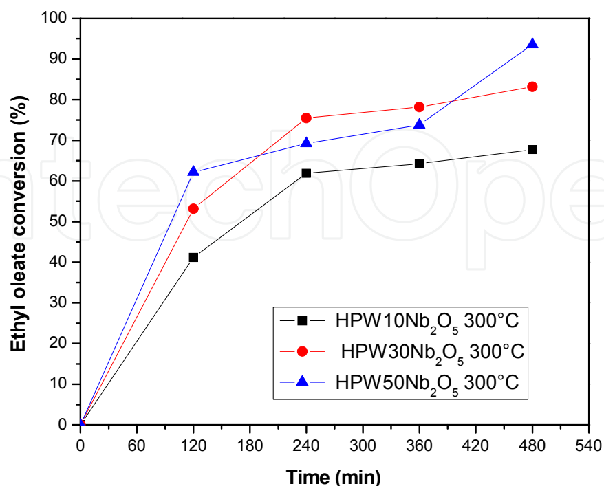
Fig. 9. Effect of the HPW load on HPW/ \text{Nb}_2\text{O}_5 -300 °C-catalyzed oleic acid esterification with ethanol
