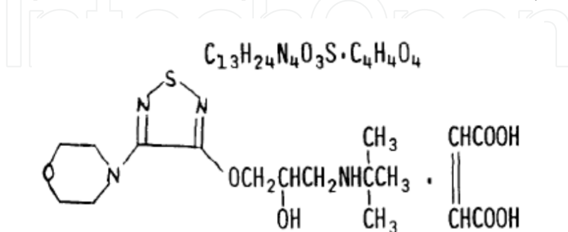
Fig. 1.0. Chemical structure and formula of timolol maleate
