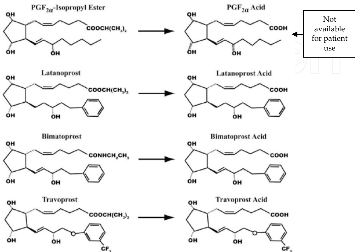
Fig. 1.2. Chemical structure of major topical prostaglandin analogue pro-drugs and their hydrolyzed free acids.
