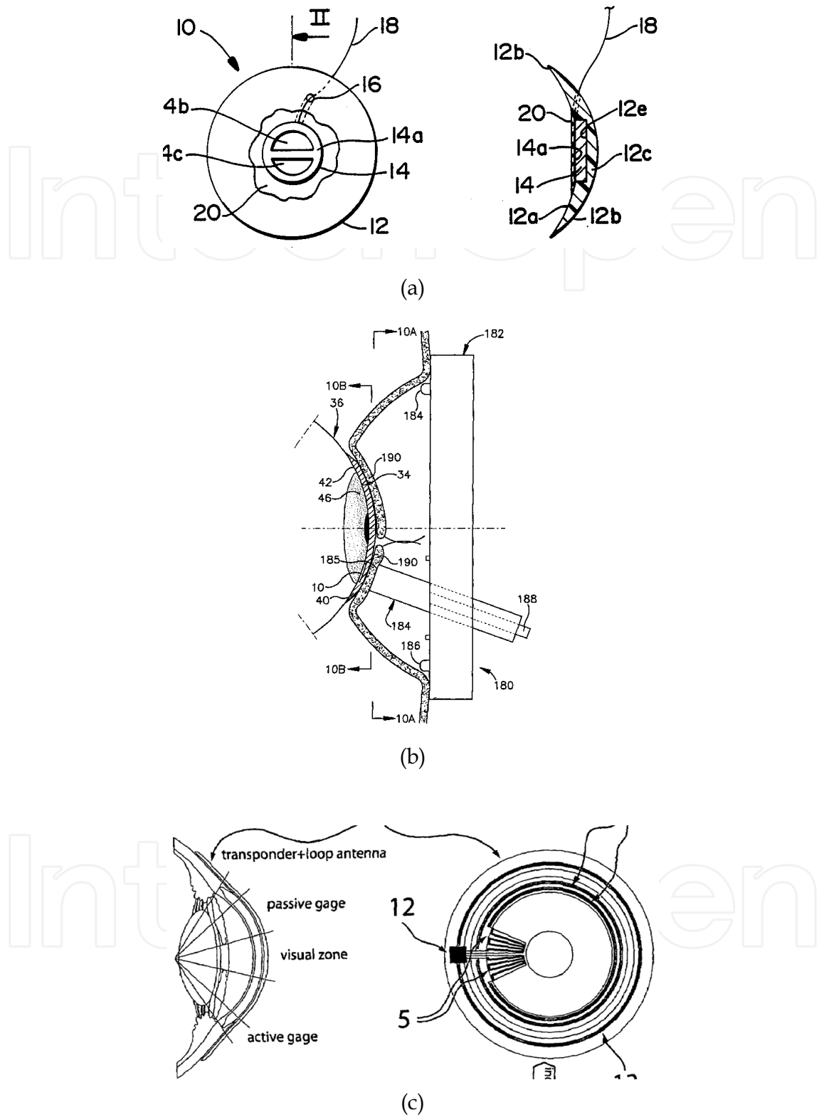
Fig. 16. IOP measurement techniques with pressure sensors on corneal contact lens (a) A contact lens device with a flat back and vision obstruction (Waters et al, 1990) (b) A cornea-mounted IOP sensor activated by a plunger (Fleischman et al, 2007) (c) A contact lens with IOP measurement sensor and an unobstructed visual zone (Leonardi et al, 2004)
