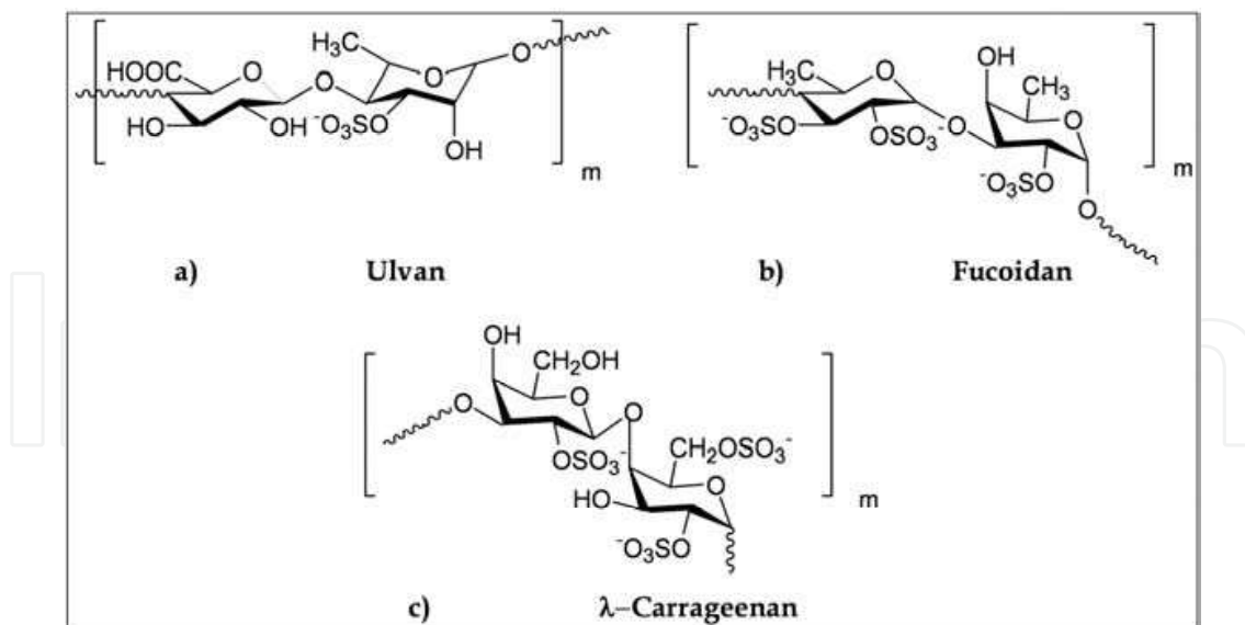
Fig. 1. Chemical structure of the dimeric repeating unit of a) Ulvan, b) Fucoidan, c) \lambda -Carrageenan.
