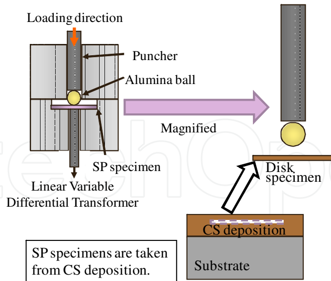
Fig. 10. Schematic illustration of small punch test
