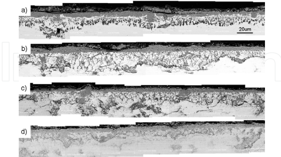
Fig. 34. Cross-sectional images of oxide layer formed at 900°C for 500h; a) substrate, b) as-sprayed, c) NHT, and d) HHT
