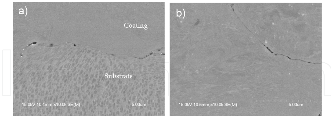
Fig. 17. Cross-sectional micrographs of the as-sprayed CS coatings showing a) the coating/substrate interface and b) near the interface
