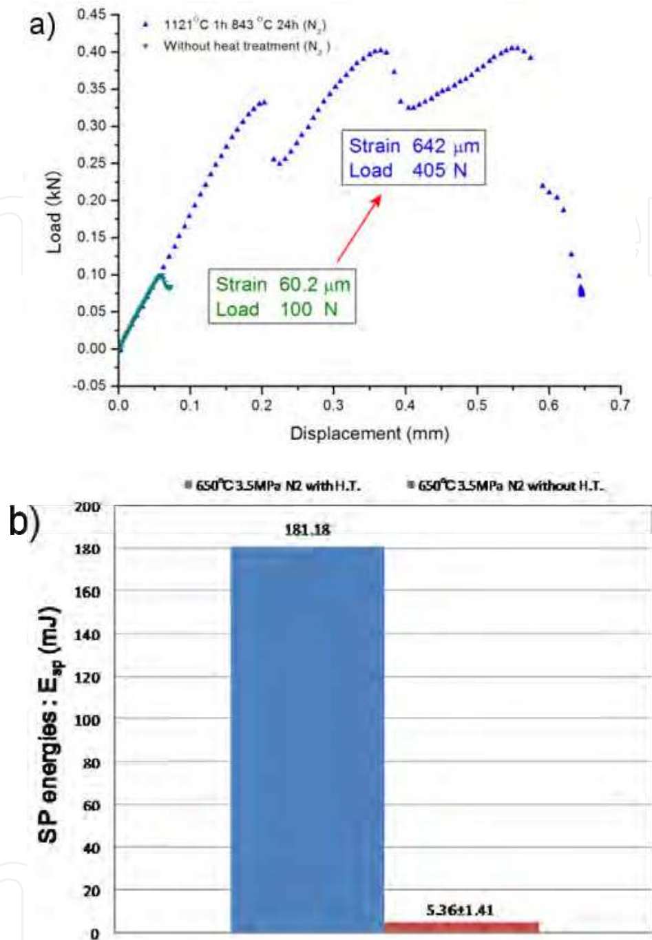
Fig. 39. Comparison of a) p-δ curves and b) SP energy with and without PSHT
