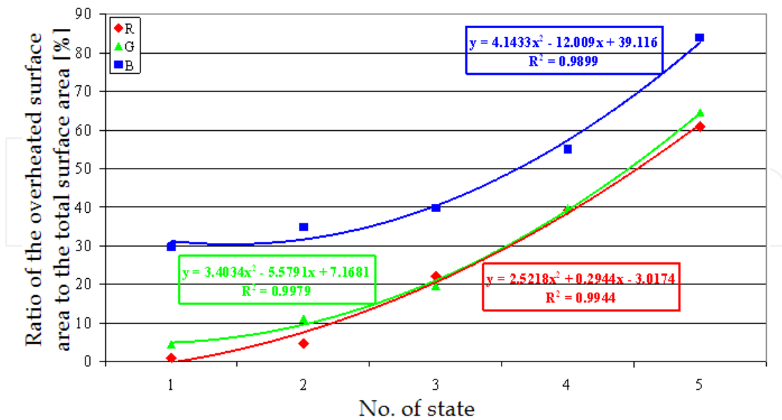
Fig. 26. Ratio of the overheated surface area to the overall surface area –images recorded with a digital photo camera
