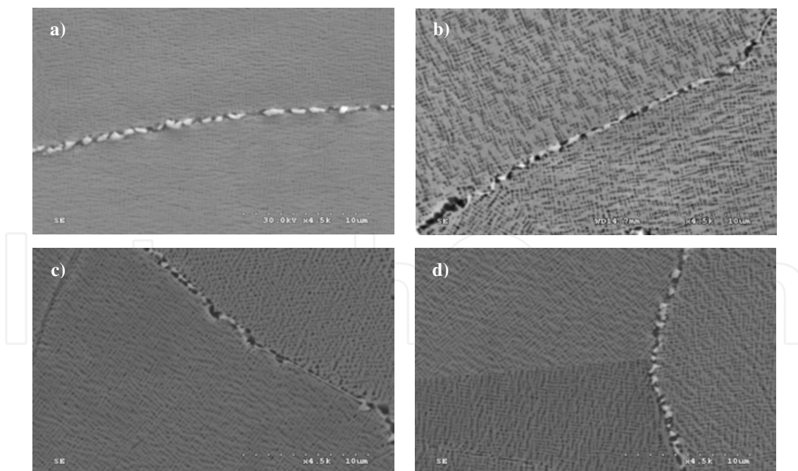
Fig. 2. Morphology of \gamma' precipitates – soaking at temperature 1223 K over: a) 0.5 h, b) 1 h, c) 2 h, d) 3 h (magn. \times 4500 )
