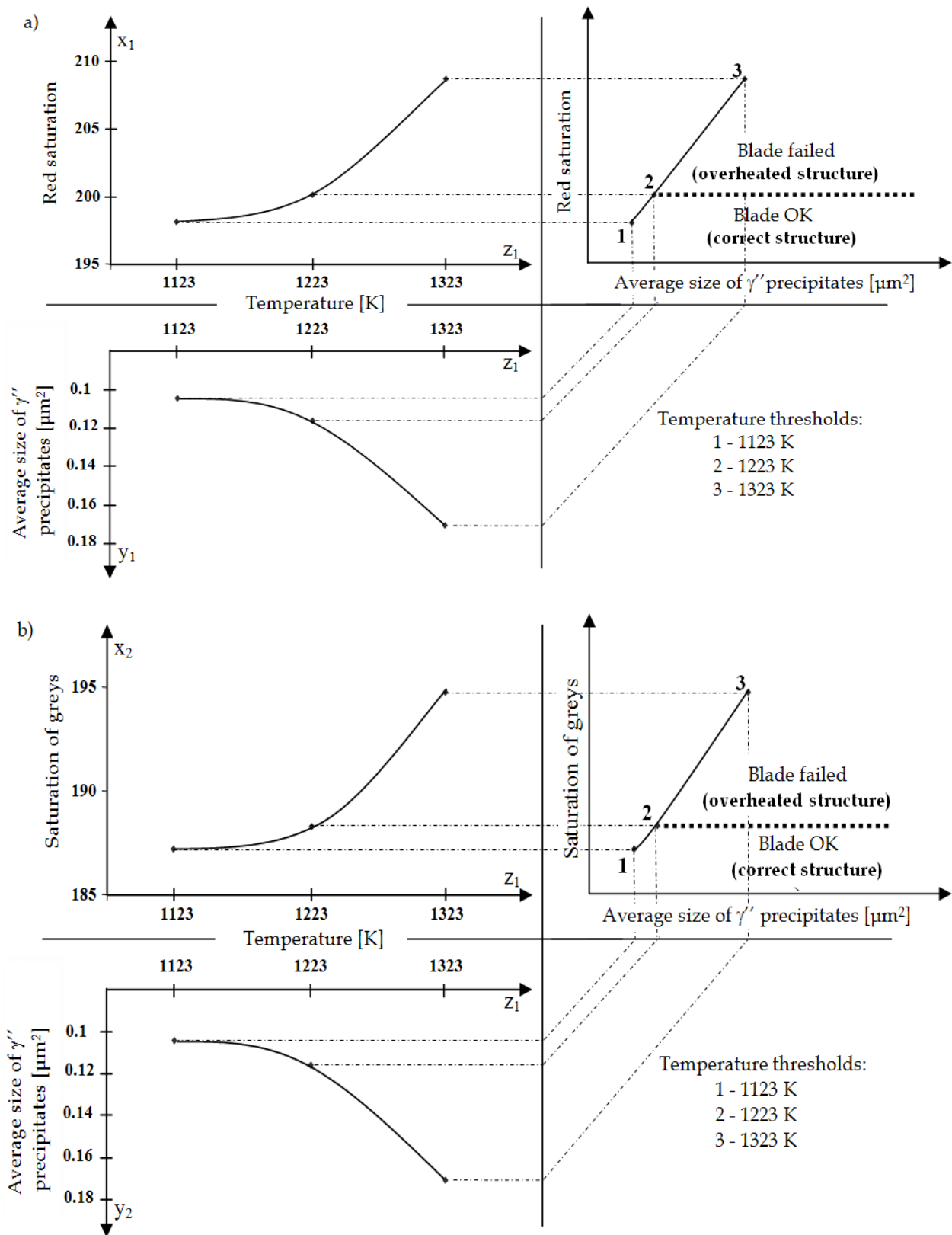
Fig. 14. Nomogram for the assessment of health of gas turbine blades on the basis of a) – alteration in Red saturation, b) – changes in shades of grey, as affected with changes in \gamma'' precipitates at different temperatures of blade soaking
