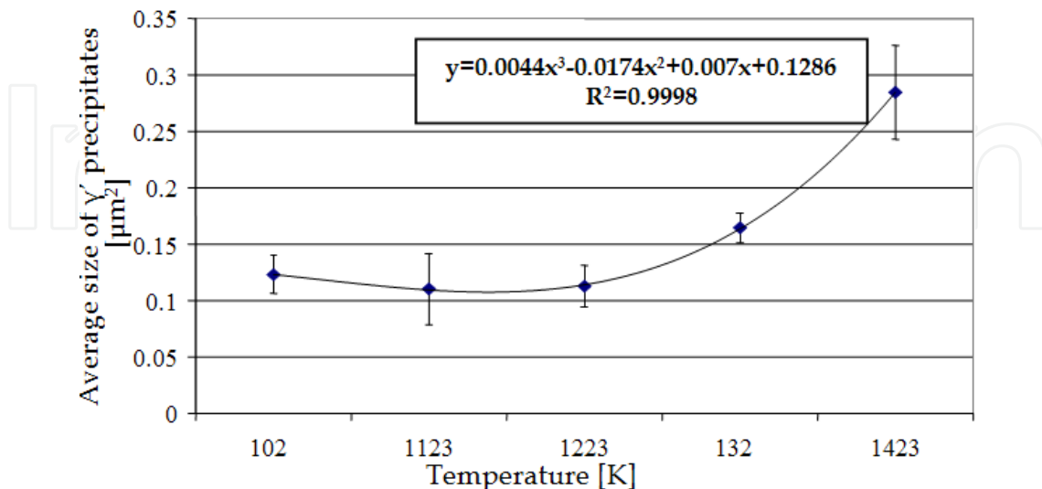
Fig. 12. Variation in \gamma' particles of average size against temperature
