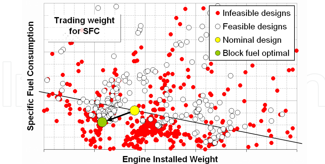
Fig. 8. Visualization example of constrained design space exploration.
