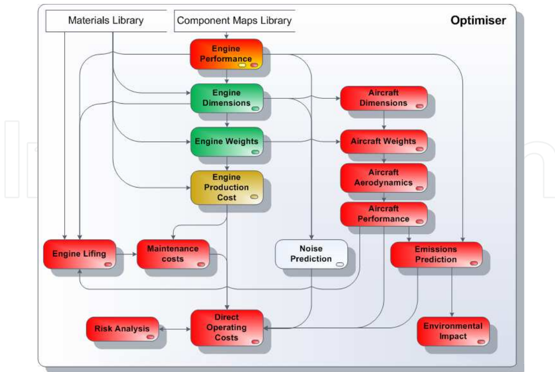
Fig. 5. Conceptual design tool algorithm (Kyprianidis, 2010).
