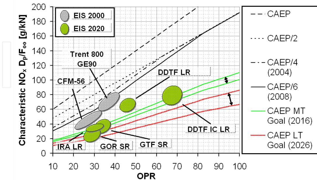
Fig. 11. NO x emissions assessment for different future aero engine design concepts.
