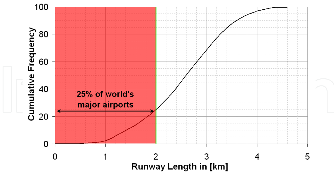
Fig. 7. Cumulative distribution of world's major runway lengths (based on data from Jenkinson et al. (1999)).
