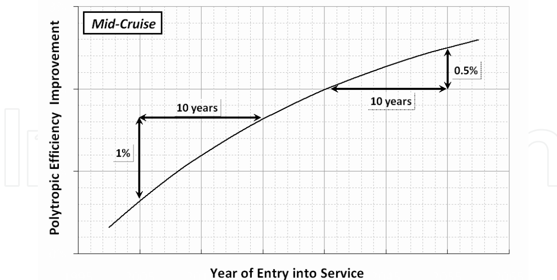
Fig. 2. Compressor efficiency improvement with year of entry into service.
