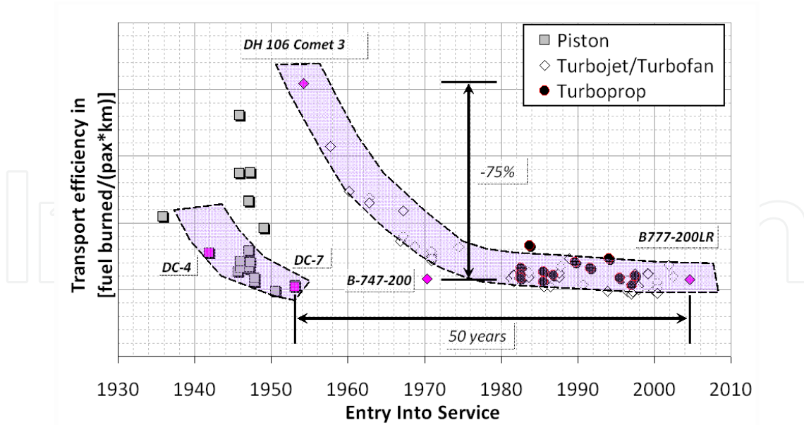
Fig. 9. Evolution of aircraft transport efficiency (based on data from Avellán (2008)).
