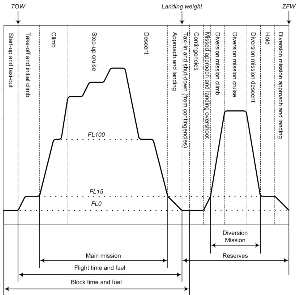
Fig. 6. Typical flight cycle.
