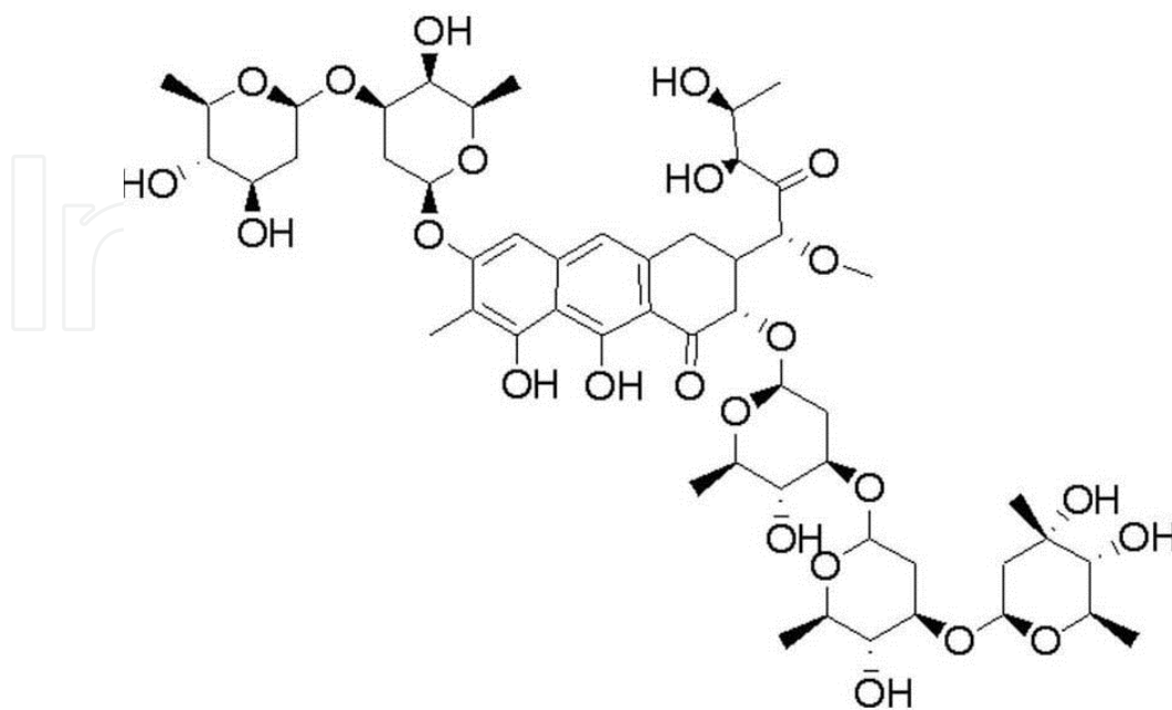
Fig. 2. Chemical structure of mithramycin [from sigmaaldrich]
