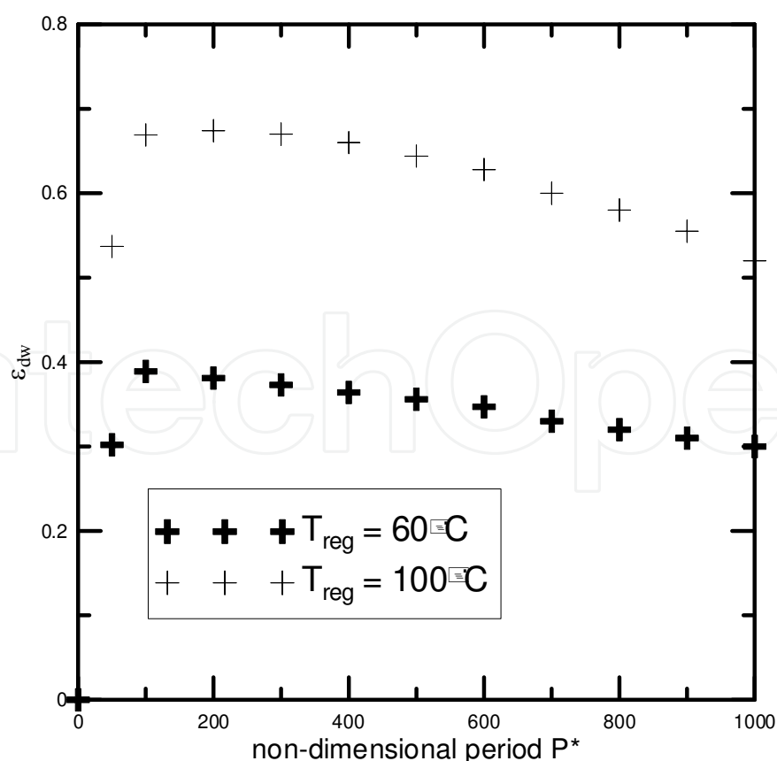
Fig. 12. Influence of P^* , NTU=10.0 .
