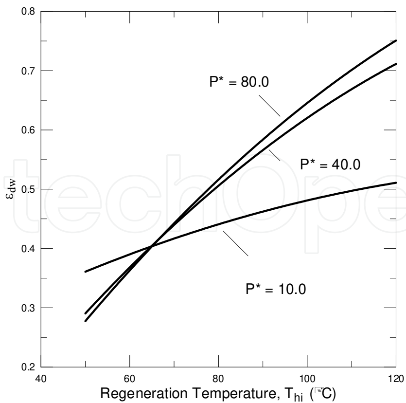
Fig. 11. Influence of P^* , NTU=10.0 , T_{hi} = 100^\circ C
