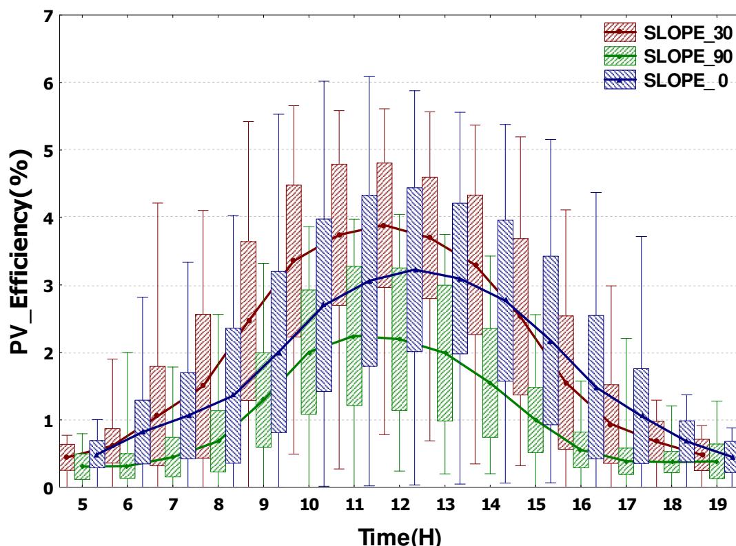
Fig. 19. Annual hourly averaged power efficiency
