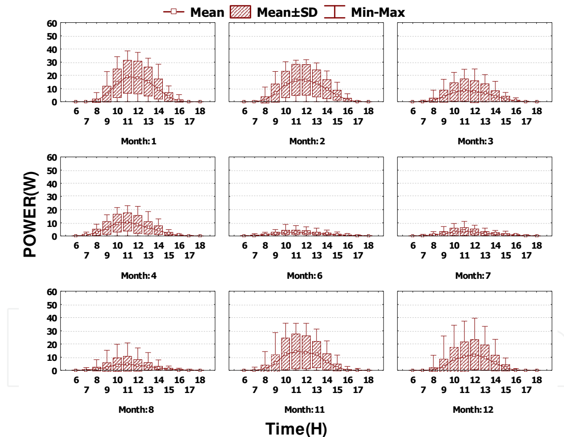
Fig. 10. Power generation of SLOPE. 90^\circ in each timestep
