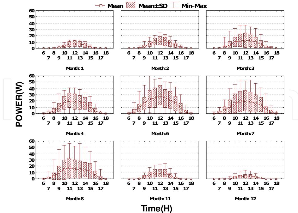
Fig. 12. Power generation of SLOPE_0° in each timestep
