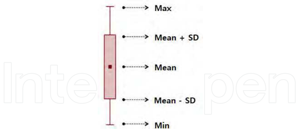
Fig. 9. Explanation of Box-Whisker graph
