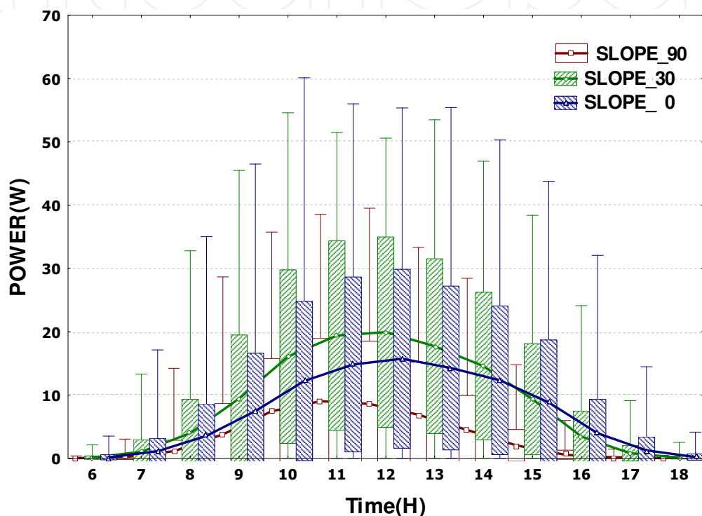
Fig. 13. Annual hourly averaged power generation
