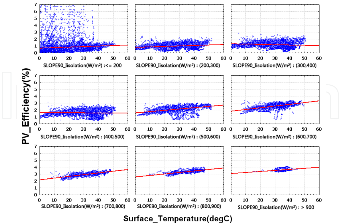
Fig. 21. Correlation between the surface temperature and power efficiency (SLOPE_90°)
