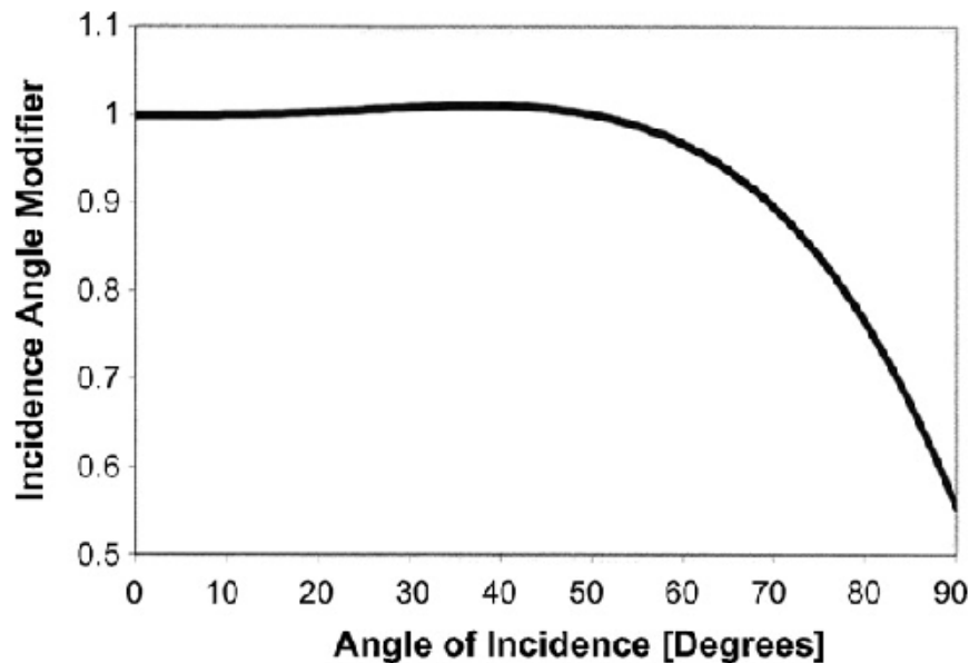
Fig. 18. Correlation of incidence angle modifier given by King et al. (1994).
