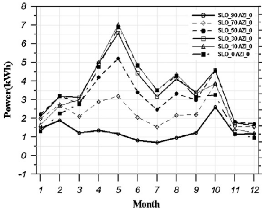
Fig. 15. Monthly power output data of PV module depending on the slope, and facing south (azimuth = 0).
