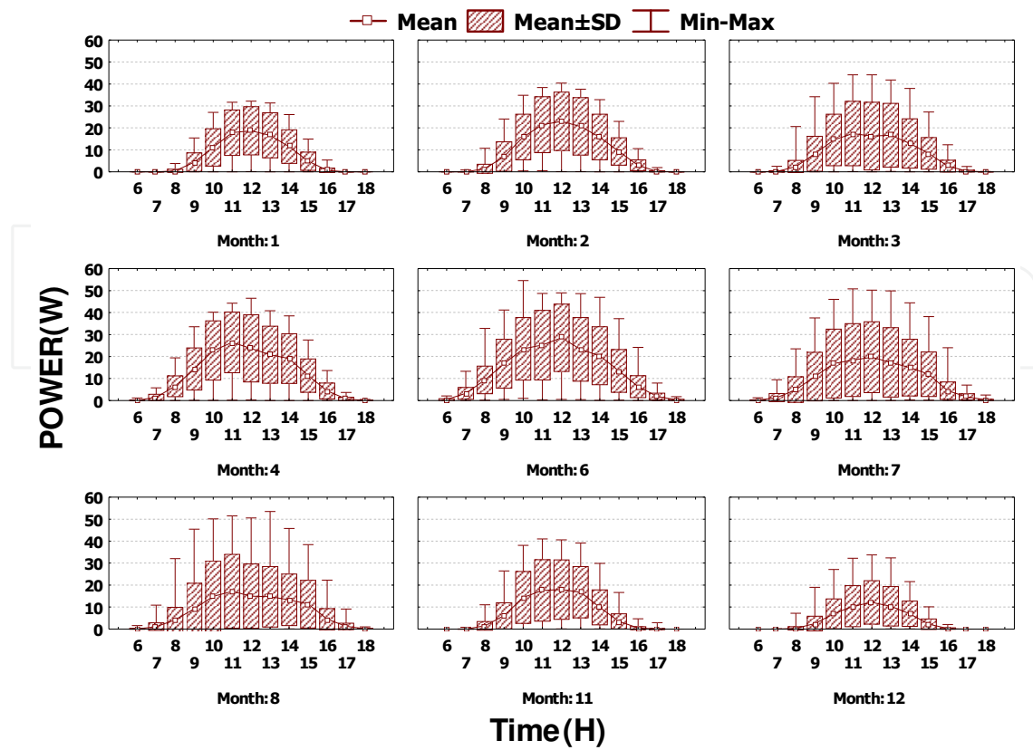
Fig. 11. Power generation of SLOPE_30° in each timestep
