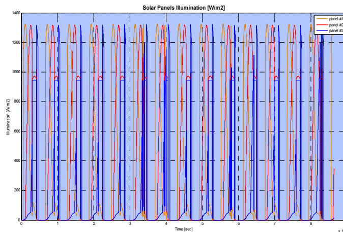
Fig. 22. Illumination of solar panels over 24 hours period
