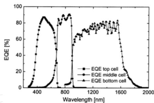
Fig. 2. Equivalent quantum efficiency as function of wavelength
