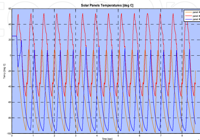
Fig. 23. Temperature of solar panels over 24 hours period
