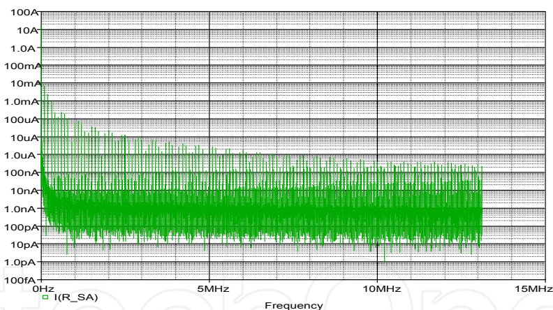
Fig. 16. Frequency Spectrum of Solar Array output current for MPPT power conditioning
