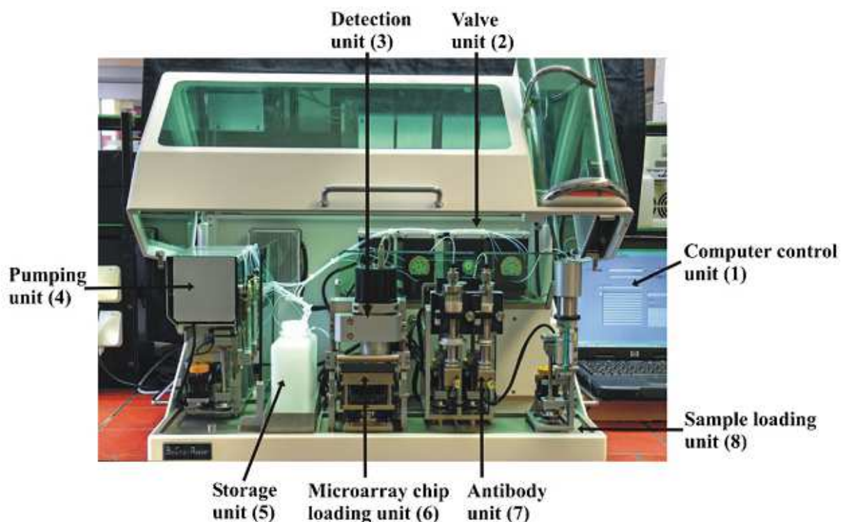
Fig. 7. Image of the MCR 3 system. Reprinted from ref. 20 with permission by the Royal Society of Chemistry.
