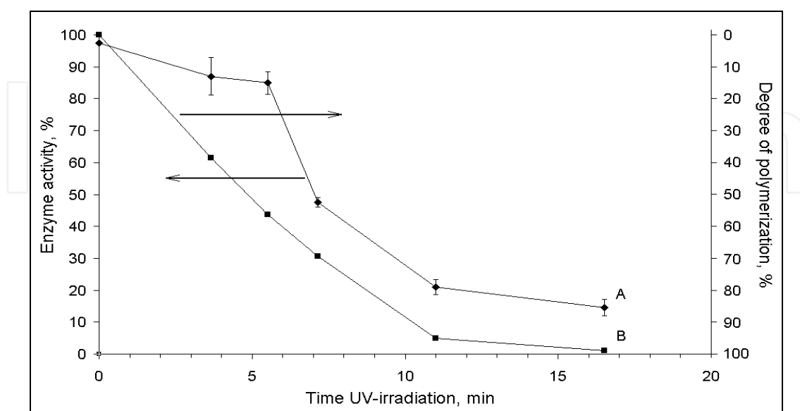
Fig. 5. Dynamics of changing in urease activity in dependence on time of UV irradiation by LUF lamp.
