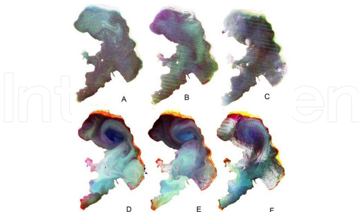
Fig. 12. Seasonal changes of Macro Prespa lake shown on the Landsat images of the year 2010: A. 14 / November B. 4 / April C.7 / June & D./ E./F. 2 / 18 / 26 of August respectively.
