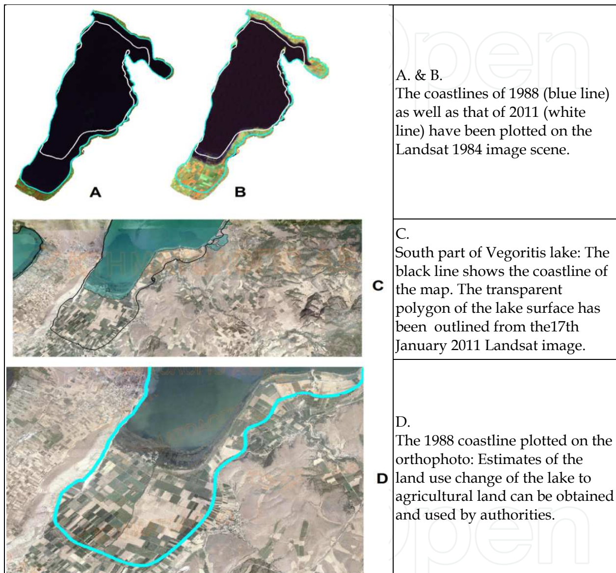
Fig. 10. Changes of the Vegoritits lake surface area.
