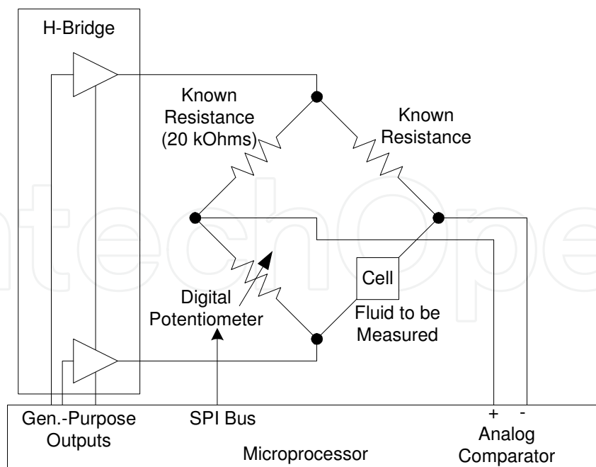
Fig. 19. Final salinity circuit.
