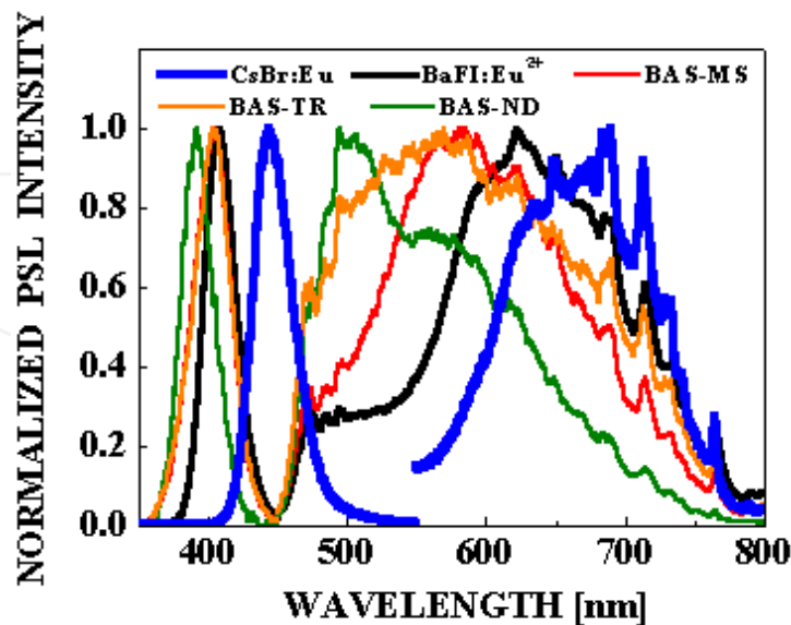
Fig. 4. OSL spectra and its stimulation (excitation) spectra of various imaging plates. Here, the IP, type-BAS-MS using BaFBr:Eu photostimulable phosphor is commercially available from Fuji Film Corp.
