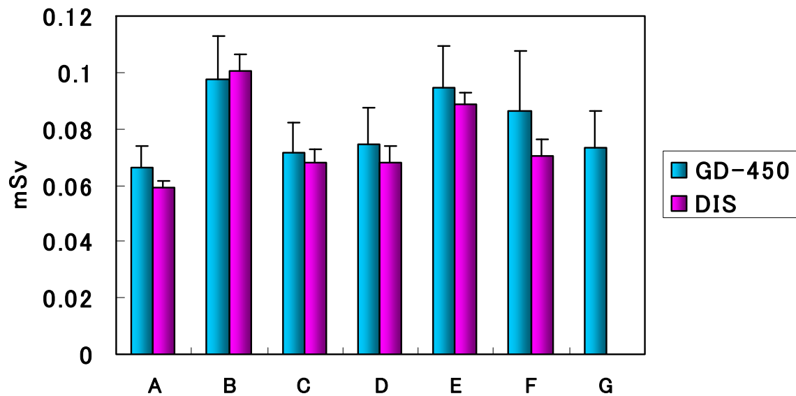
Fig. 18. Dose response at each point in Ishikawa prefecture (A: Tsurugi-machi, B: Tatsunokuchi, C: Inside of house of Mt. Shishiku, D: Outside of Mt. shishiku, E: Inside of Ogoya Mines, F: Outside of Ogoya Mines, G: Public health and Environmental Science) using GD-450 (blue bars) or DIS (purple bars) dosimeters. There is no data at G for DIS.
