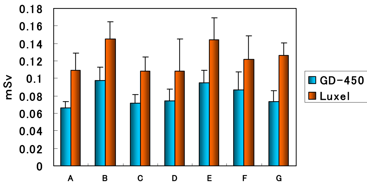
Fig. 17. Dose response at each point in Ishikawa prefecture (A: Tsurugi-machi, B: Tatsunokuchi, C: Inside of house of Mt. Shishiku, D: Outside of Mt. shishiku, E: Inside of Ogoya Mines, F: Outside of Ogoya Mines, G: Public health and Environmental Science) using GD-450 (blue bars) or Luxel badge (orange bars) dosimeters.
