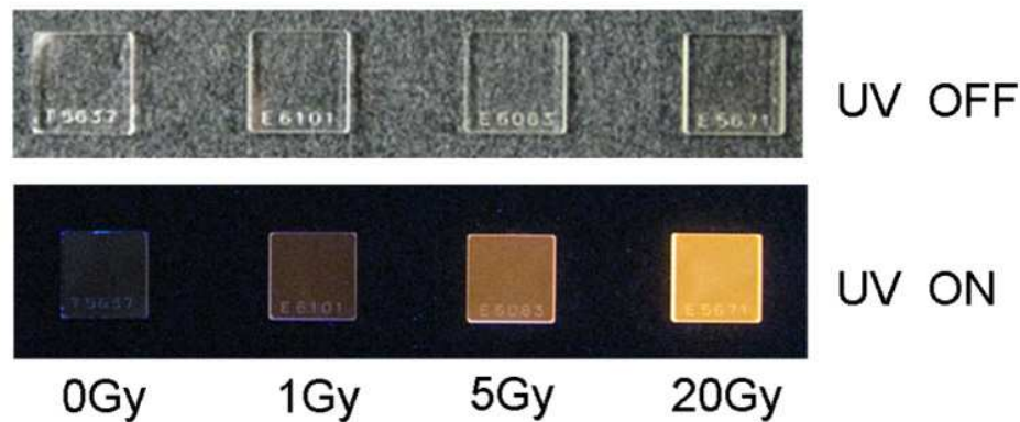
Fig. 12. RPL emission images of Ag + -doped phosphate glass as a function of x-ray absorbed dose : (a) Ag + -doped phosphate glass under visible light, (b) Ag + -doped phosphate glass under UV light.
