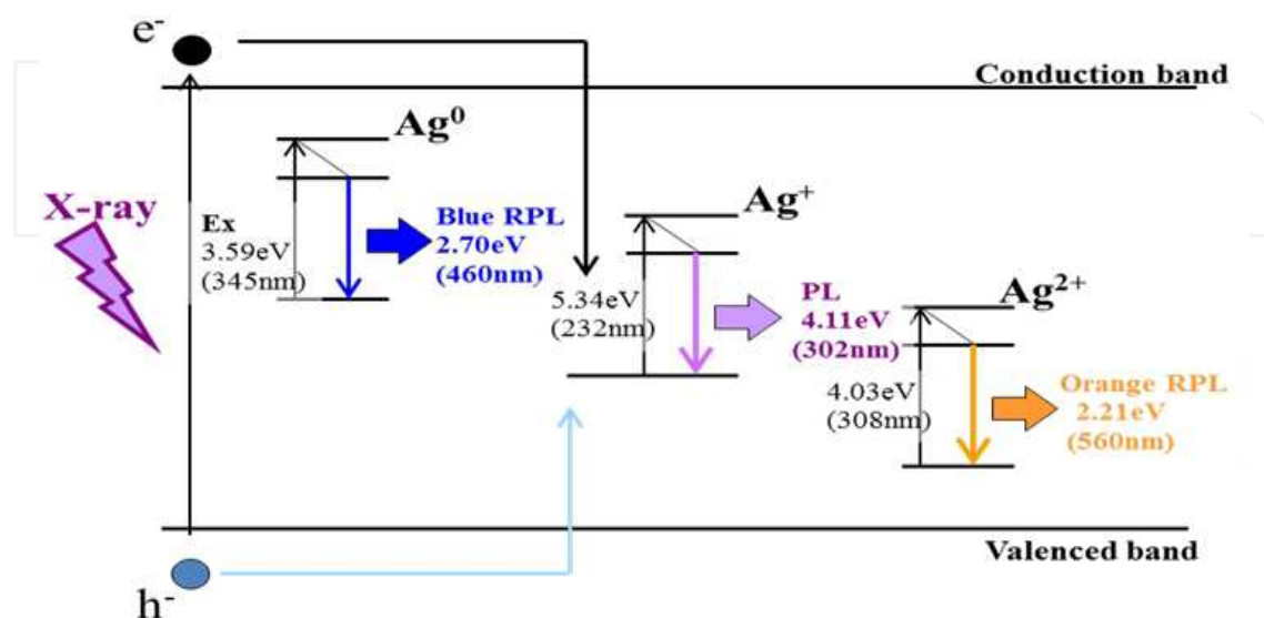
Fig. 1. Energy band diagram for RPL centers in \text{Ag}^+ -doped phosphate glass.
