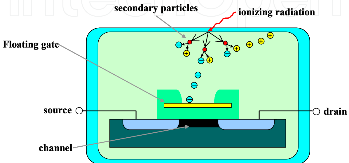
Fig. 5. Schematic diagram of the DIS dosimeter
