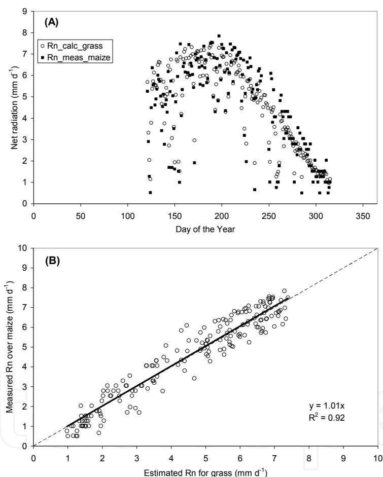
Fig. 12. (A) Comparison of daily net radiation ( R_n ) measured over maize ( R_n\_meas\_maize ) with R_n calculated for grass ( R_n\_calc\_grass ) using the procedure described in FAO-56 (1998), and (B) regression analysis of measured and estimated R_n data in (A) (— Linear regression line, ---1:1 line, n = 185 ).
