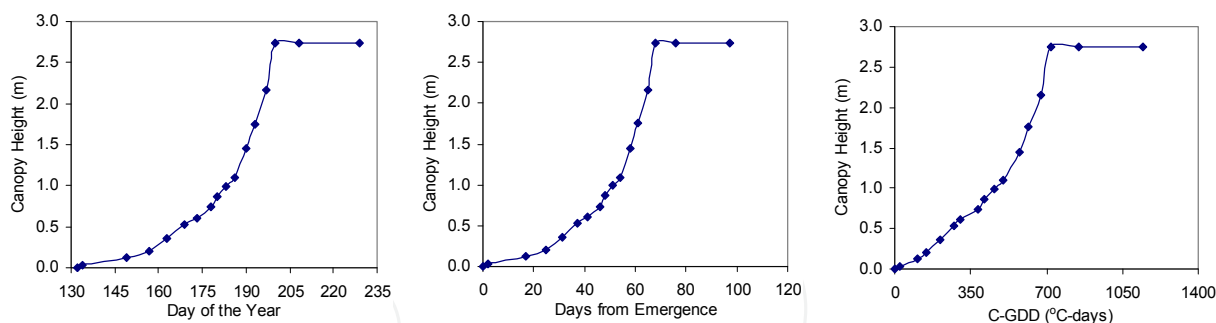
Fig. 5. Maize canopy height as a function of day of the year, days from emergence, and cumulative growing degree days from emergence (C-GDD) measured at North Platte, Nebraska, during the 2001 growing season. Daily growing degree days were calculated using a lower limit (base temperature) of 10 °C (50 °F), with no upper limit imposed.
