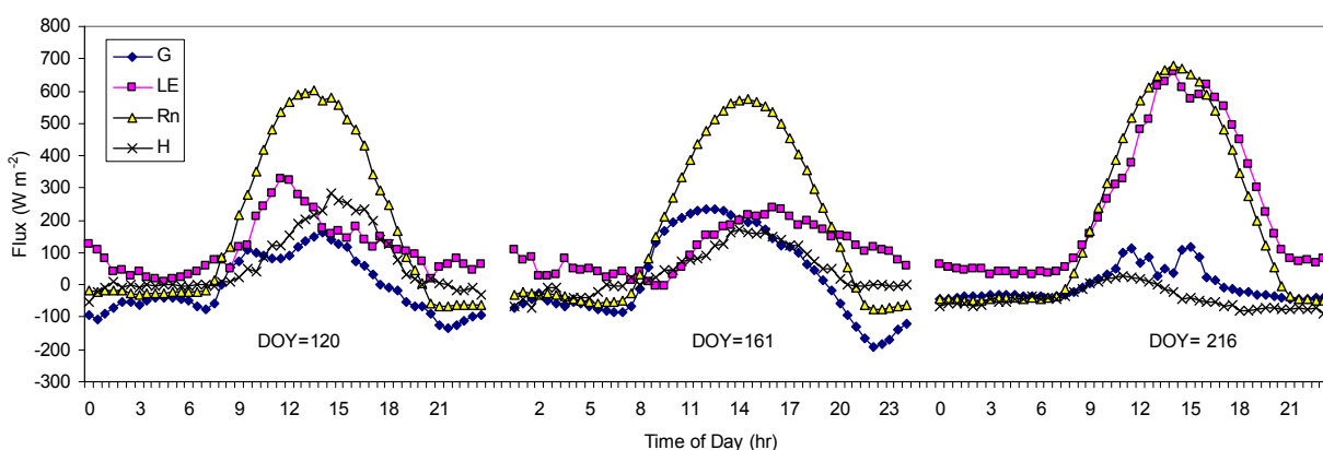
Fig. 10. Values of energy balance components measured during three clear-sky days on a surface-irrigated maize field at North Platte, Nebraska, during 2001. LE = latent heat flux (ETc), H = sensible heat flux, G = soil heat flux, Rn = net radiation. Each data point represents the 30-min average flux. DOY =day of the year. Maize was planted on DOY 128.
