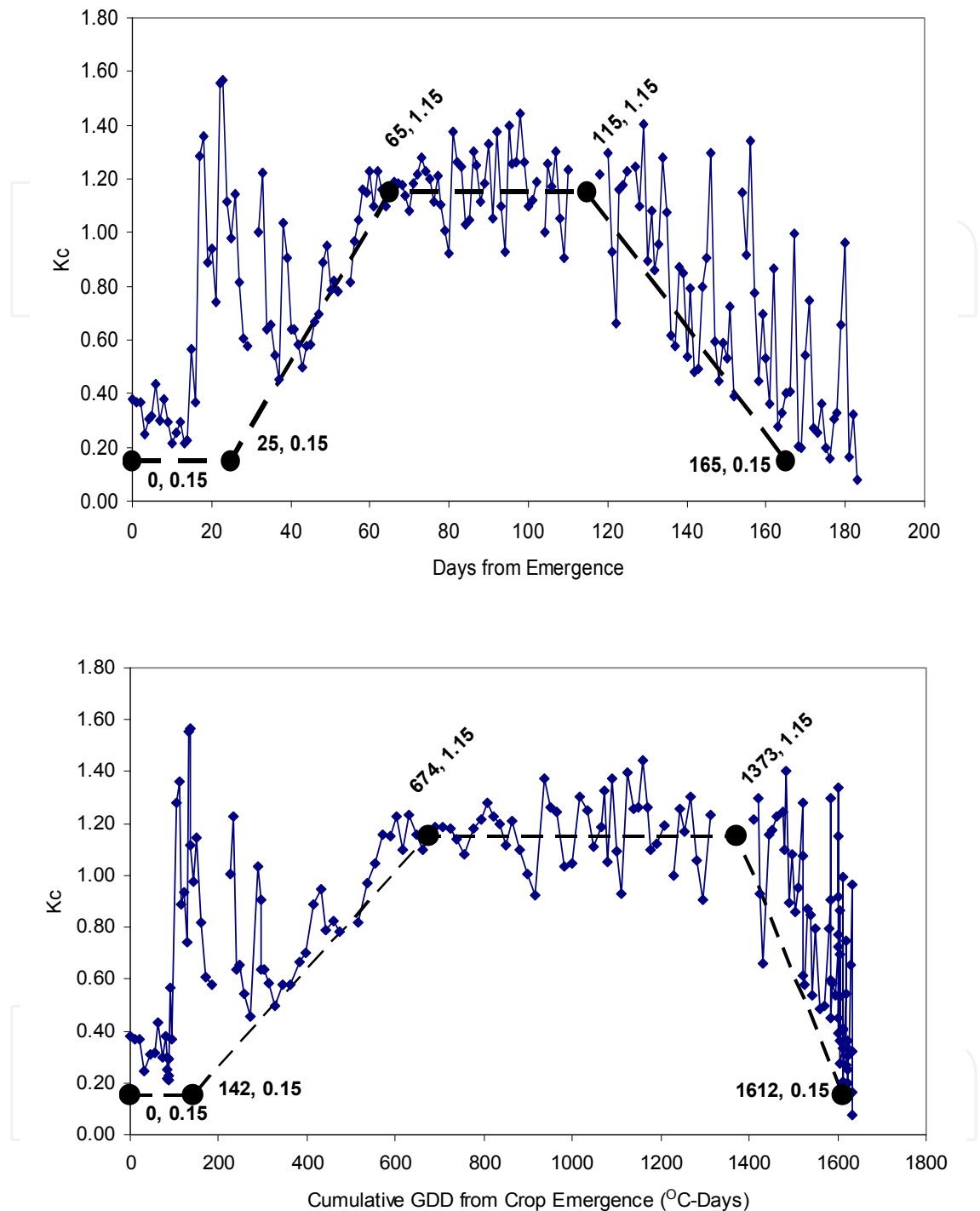
Fig. 14. Crop coefficient ( K_c ) curves for field maize measured at North Platte, Nebraska, during 2001, as a function of days from emergence and cumulative growing degree days (GDD) from crop emergence. The K_c values were calculated based on a grass reference ( E_{To} ), which was calculated with the FAO-56 method. The broken line represents the K_c function proposed in FAO-56 with growth stage lengths for Kimberly, Idaho. The number pairs on the graphs are the coordinates for each of the black dots for the Kimberly curves from FAO-56 ( n = 182 ).
