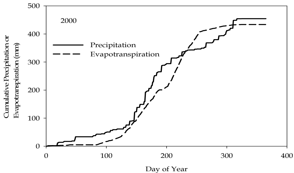
Fig. 4. Annual cumulative precipitation and evapotranspiration for a corn production field for Central Iowa in 2000.
