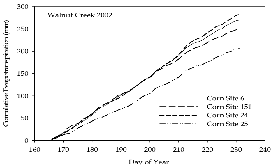
Fig. 7. Cumulative evapotranspiration across four corn fields with detailed measurements in Walnut Creek watershed in 2002.
