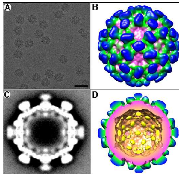
Fig. 4. CryoEM structure of the large VLPs. (A) CryoEM micrographs of large VLPs embedded in vitreous ice (Bar=1000 Å). (B) Shade surface of the large VLP reconstruction at about 11 Å resolution as viewed along the twofold axis (Electron Microscopy Data Bank accession number: EMD-5173). Different domains are colored differently, the S domain colored magenta, P1 domain green, P2 domain blue. (C) A central slice view along the twofold axis. (D) Shaded surface representation of the 3D reconstruction after its upper half was removed to reveal the internal view; the N domain is colored yellow.
