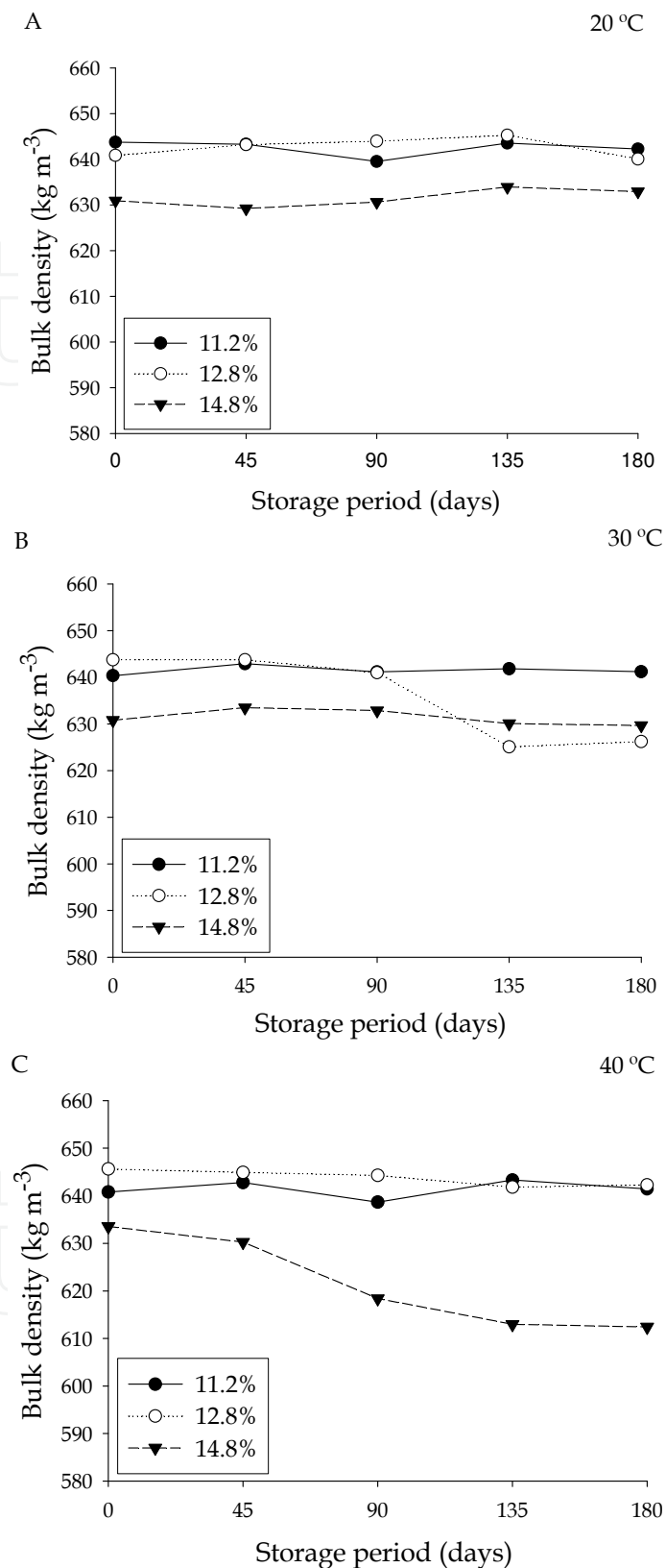
Fig. 1. Average measurements of bulk density for soybeans stored with moisture contents of 11.2, 12.8 and 14.8% (w.b.) at the temperatures of 20, 30 and 40 °C.
