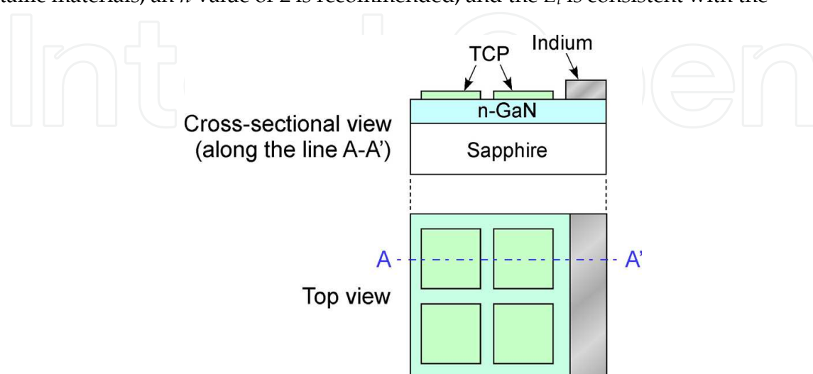
Fig. 2. Schematic of TCP/epi.-GaN sample.
