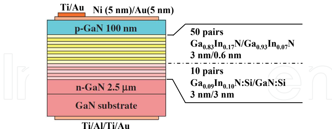
Fig. 1. Schematic of In x Ga 1-x N-based solar cell exhibiting 2.5% conversion efficiency (Kuwahara, 2011).
