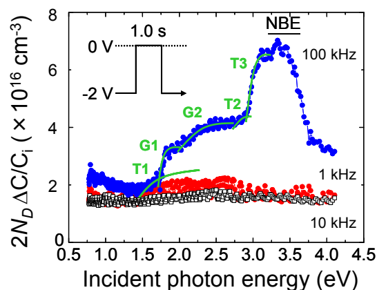
Fig. 7. DLOS spectra of PANI/epi.-GaN heterojunction solar cell.
