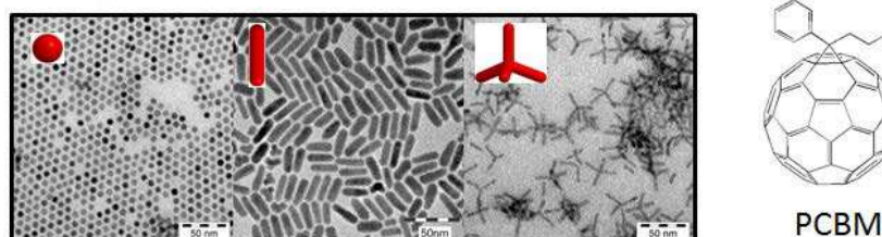
Semiconductor Nanocrystals
