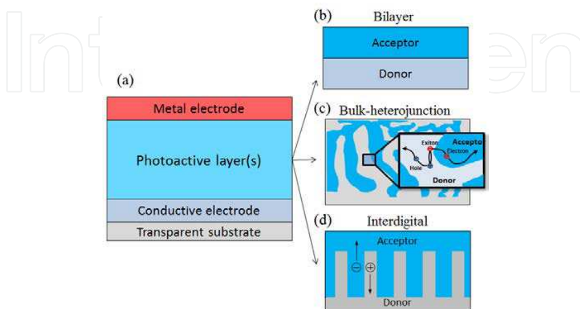
Fig. 1. Schematic illustration of typical device structures for hybrid solar cells.
