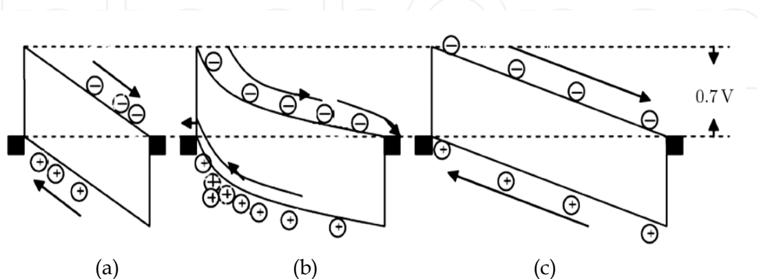
Fig. 2. Energy band diagrams under short circuit condition. (a) Case I: thickness is shorter than both drift lengths, (b) Case II: thickness is longer than hole drift length but shorter than electron drift length, (c) Case III: thickness is longer than both hole and electron drift lengths.
