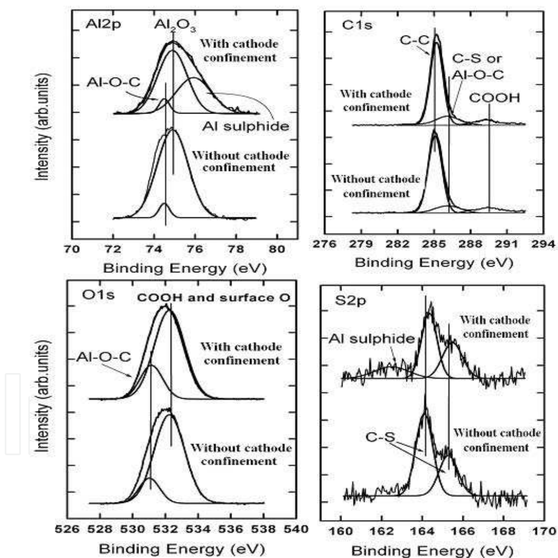
Fig. 10. High-resolution Al 2p, C 1s, O 1s and S 2p XPS spectra of the samples without (bottom curve) and with (top curve) the cathode confinement in the thermal treatment. The samples have the configuration of ITO/P3HT:PCBM (100 nm)/ Al(3 nm). By using the cathode confinement, there is an additional shoulder peak at the BE of 76 eV in the Al 2p spectrum and an additional shoulder peak at the BE of 162.4 eV in the S 2p spectrum.
