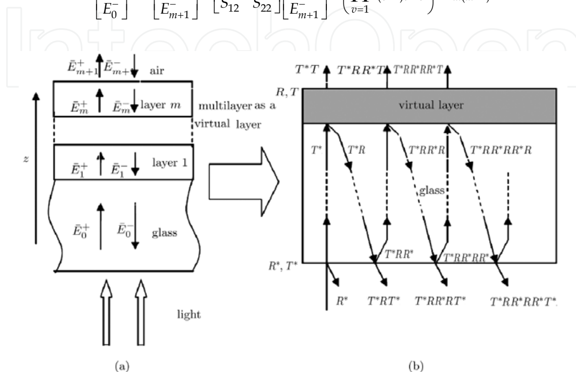
Fig. 1. Multilayer structure in a polymer solar cell. (a) the optical electric field in each layer and (b) treating the multilayer as a virtual layer.
