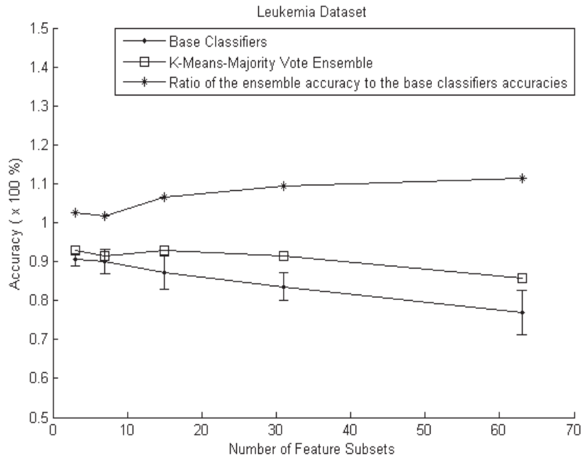
Fig. 7. Results of the k-means-majority vote ensemble.
