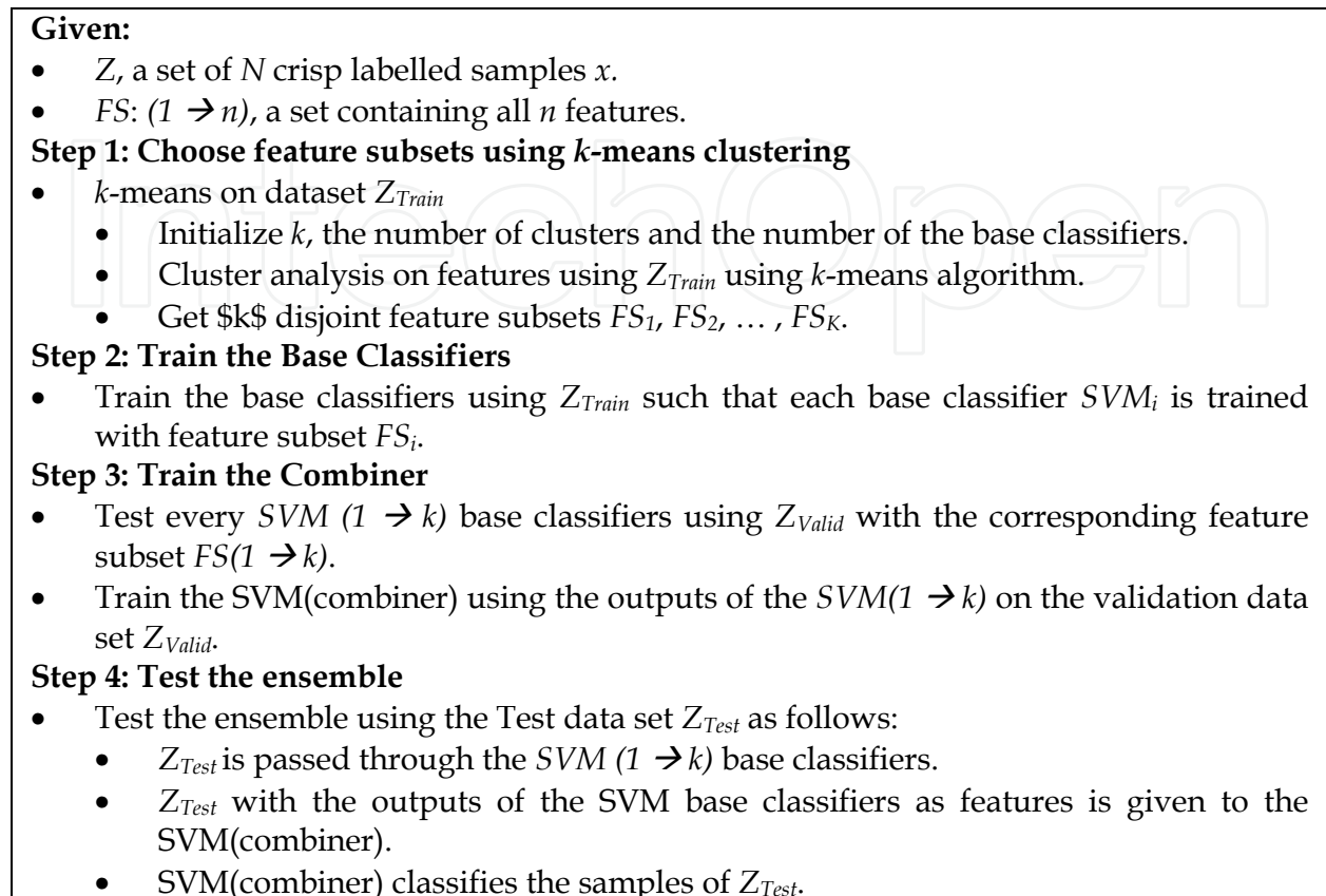
Fig. 5. Ensembles using SVM fusion.
