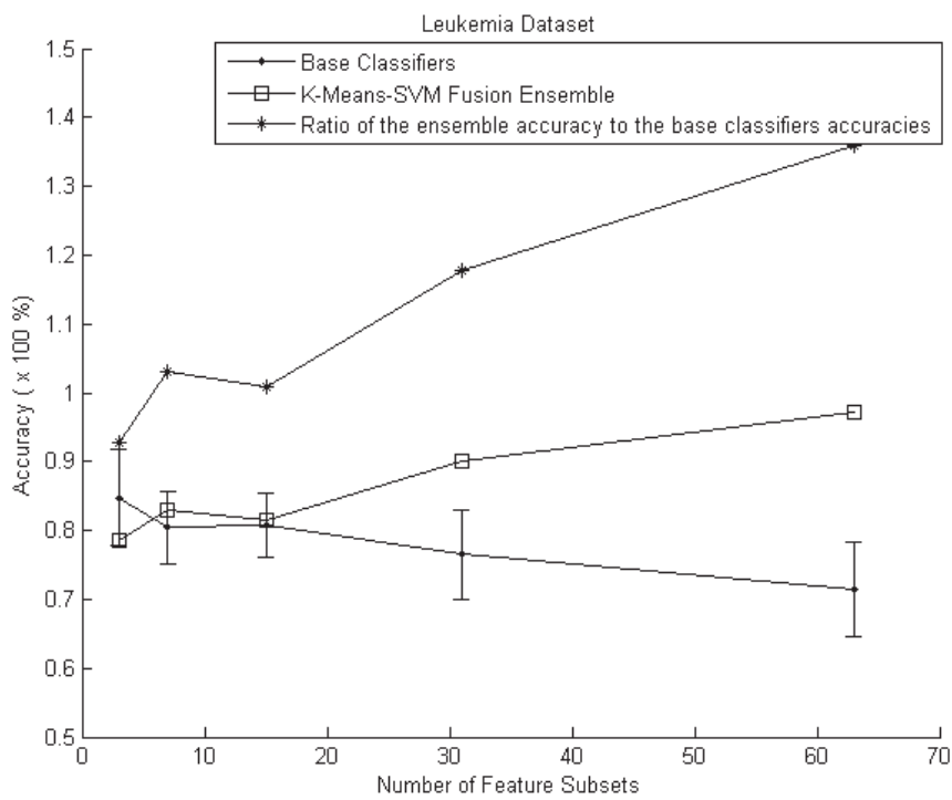
Fig. 8. Results of the k-means-SVM fusion ensemble.
