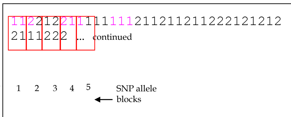
Fig. 3. Consecutive 3-SNP allele blocks along 1 row representing either a paternal or maternal chromosome.
