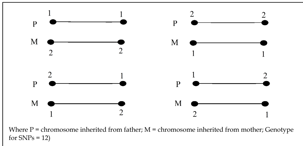
Fig. 1. Possible haplotype when 2 SNPs have heterozygous alleles.
