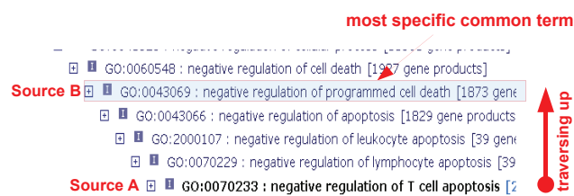
Fig. 7. Find the most specific common term by traversing up the hierarchy. (This figure shows an extract of the Gene Ontology http://www.geneontology.org )
