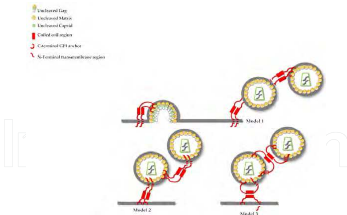
Fig. 10. Tetherin-induced inhibition of HIV-1 particle release. Each model centres on the dimerization of two tetherin molecules. In model 1, the N-terminal transmembrane regions of the tetherin dimer anchor to the cell surface and the C-terminal GPI domains associate with the budding virus. Model 2 is the opposite of model 1. In model 3, each tetherin molecule of the dimer associates with either only the budding virus or only the cell membrane, and HIV-1 restriction depends on the interaction between the coiled-coil regions.
