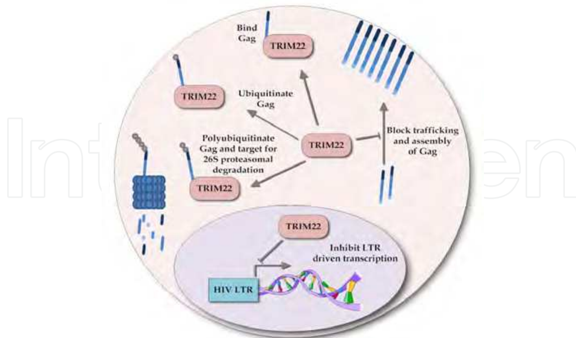
Fig. 9. Possible mechanisms of TRIM22-mediated HIV-1 restriction. TRIM22 prevents accumulation of the Gag polyprotein at the plasma membrane, and as such may bind directly to Gag. Alternatively, TRIM22 may mono-ubiquitinate or polyubiquitinate Gag. Experiments using LTR-luciferase reporter constructs have also shown that TRIM22 restricts transcription from the 5' HIV-1 LTR.
