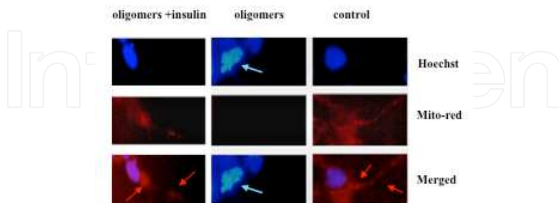
Fig. 3. Insulin recovers mitochondrial respiratory activity reduced by rAb42 oligomers. LAN5 untreated (control), treated with rAb42 oligomers (oligomers), and rAb42 oligomers and insulin (oligomers+insulin) were incubated with Mito Red and Hoechst 33258. The images of each sample were merged. Mitochondrial activity is indicated by red arrows, fragmentation of nuclei is indicated by blue arrows.
