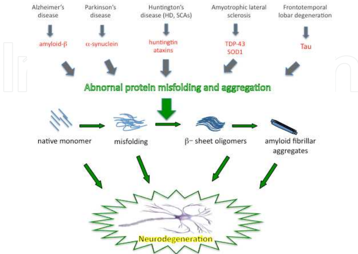
Fig. 1. Protein misfolding and aggregation as the common molecular pathogenesis of neurodegenerative diseases. Some genetic mutations responsible of neurodegenerative diseases render the causative proteins prone to misfold and to form beta-sheet-rich oligomers and amyloid fibrillar aggregates, resulting in their accumulation in the affected neurons and eventually leading to degeneration in the brain. This mechanism is retained common to a broad variety of neurodegenerative diseases, such as Alzheimer's, Parkinson's and Huntington disease, Amyotrophic Lateral Sclerosis and Frontotemporal Lobar degeneration.
