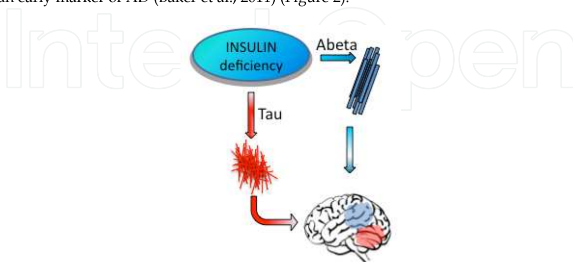
Fig. 2. Insulin deficiency can lead to Abeta plaques formation and Tau hyperphosphorylation
