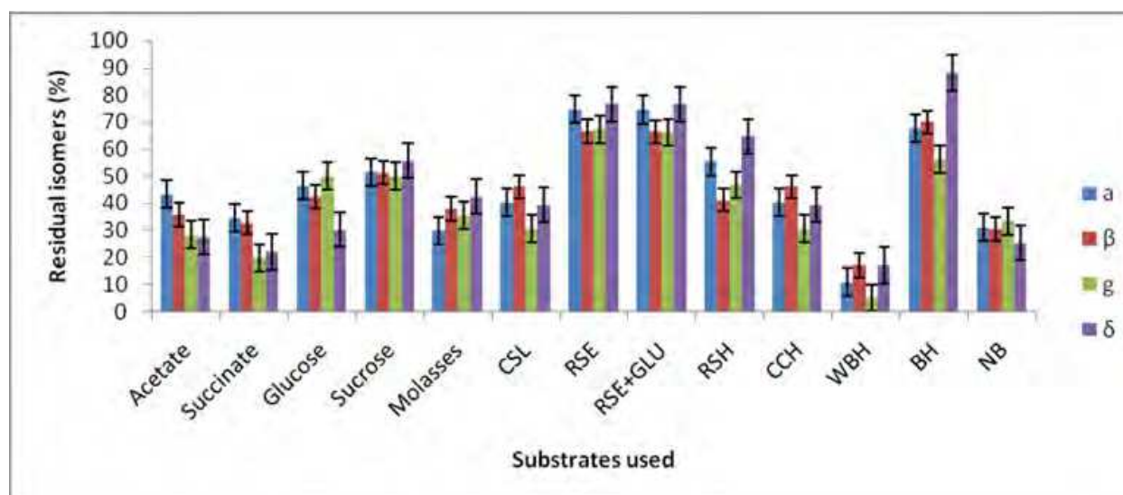
Fig. 1. Degradation of Tech-HCH with inoculum grown on different carbon sources CSL, Corn steep liquor; RSE, Rice straw extract; RSH, Rice straw hydrolysate; CCH, Corn cob hydrolysate; WBH, Wheat bran hydrolysate; BH, Bagassae hydrolysate; NB, Nutrient broth.
