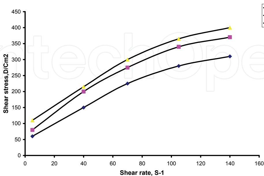
Fig. 2. Variation of shear stress with shear rate for G_{1G} , G_{2C} and G_{3D} at 120°C
