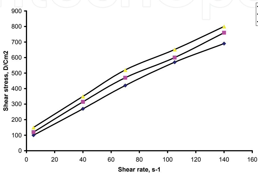
Fig. 1. Variation of shear stress with shear rate for G_{1G} , G_{2C} and G_{3D} at 90°C
