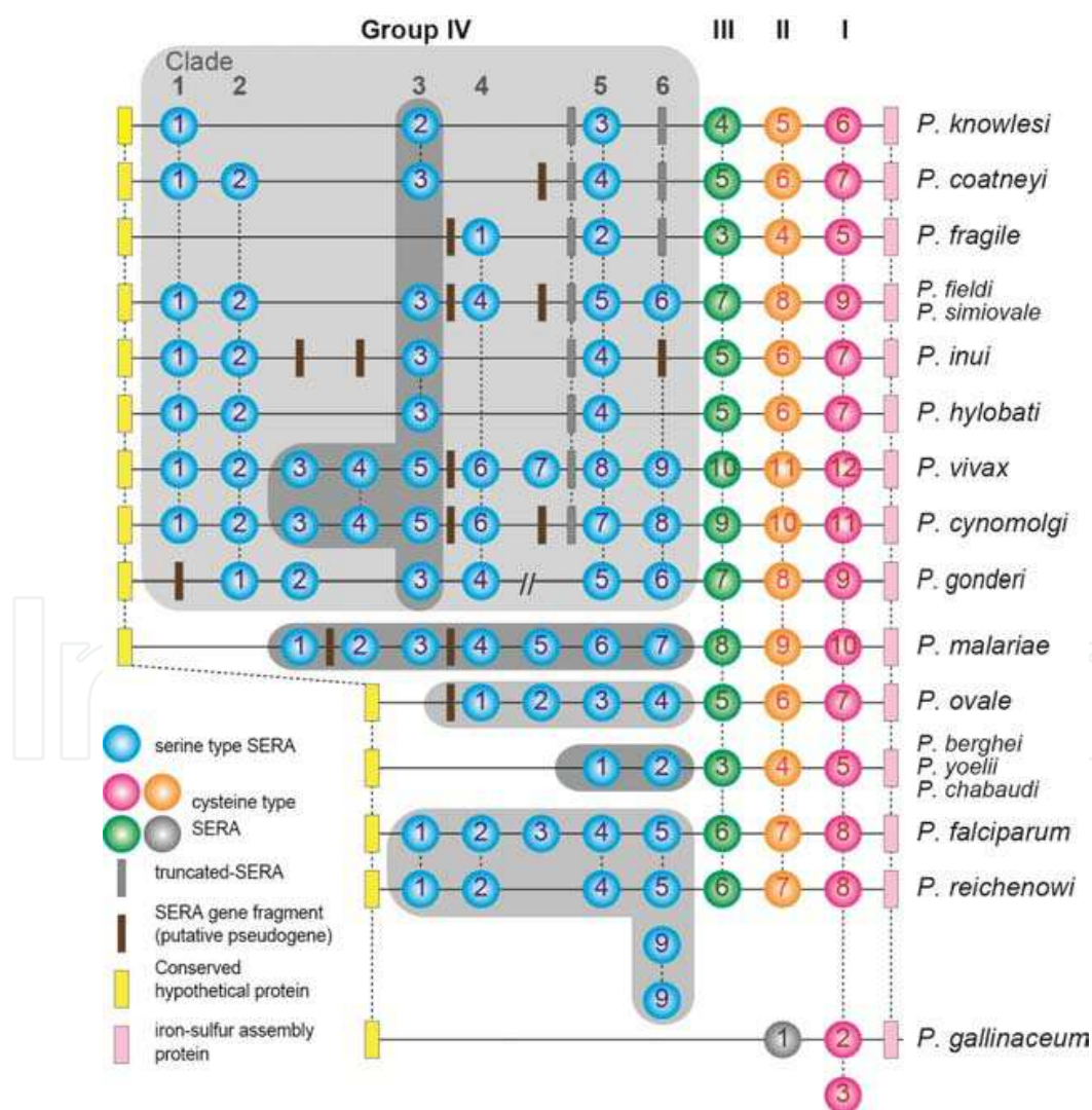
Fig. 6. Organization and phylogenetic relationship of SERA gene in 18 Plasmodium species.
