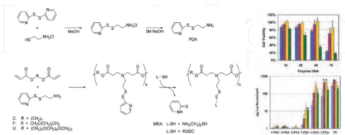
Fig. 15. Synthesis scheme of MEA (left) and cytotoxicity [C-PDA (blue), C-PDA-MEA (Redenti, et al.), 2-mercaptopyridine (2-MP, yellow), and PEI (green)] and transfection studies (right). [Source from Ref. (Zugates, et al., 2006)].
