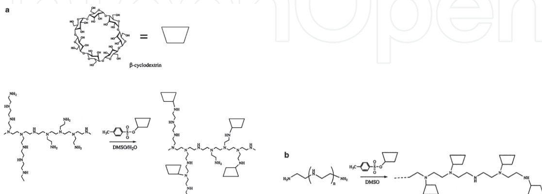
Fig. 2. (a) Synthesis of \beta -CD-bPEI. (b) Synthesis of \beta -CD-IPEI. [Source from Ref. (Pun, et al., 2004)].
