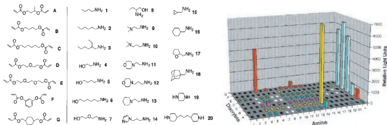
Fig. 13. Diacrylate (A-G) and amine (1-20) monomers chosen for the synthesis of an initial screening library (left) and transfection data as a function of structure for an assay employing pCMV-Luc (600 ng/well, DNA/polymer = 1:20, right). [Source from Ref. (Lynn, et al., 2001)].
