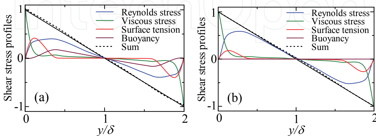
Fig. 9. Budget for shear stress.
