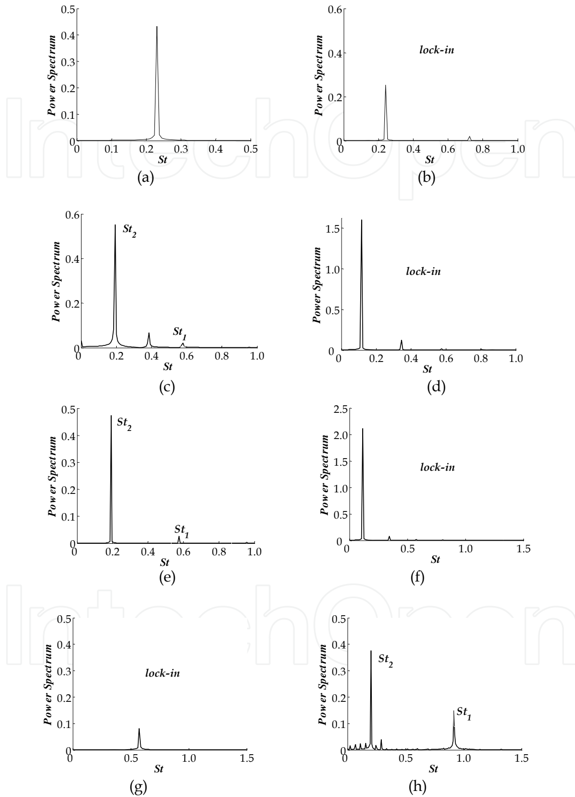
Fig. 12. Power Spectra for Re=1,000 : a) stationary cylinder; b) and c) A=1 and f_c / f_o = 1.05 and f_c / f_o = 2.5 respectively; d) and e) A=2 and f_c / f_o = 0.5 and f_c / f_o = 2.5 respectively and f) g) and h) A=3 and f_c / f_o = 0.5 , f_c / f_o = 2.5 and f_c / f_o = 4.0 respectively.
