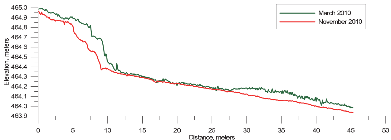
Fig. 17. User-defined centreline with Z elevation values obtained from the point of intersection with generated cross-sections for March (green) and November (red) of 2010.
