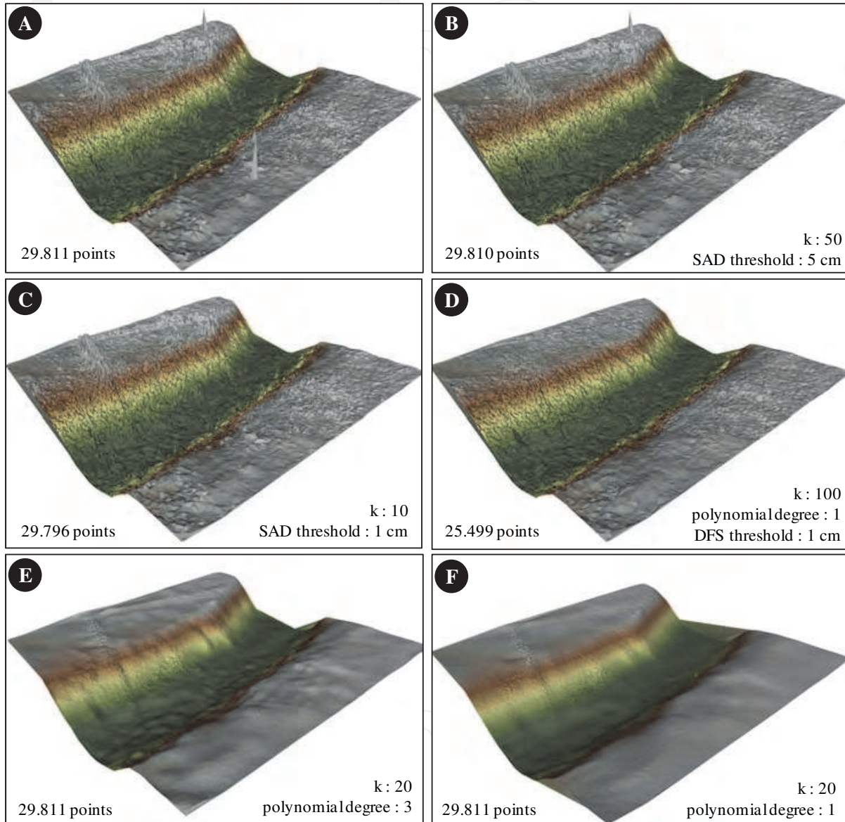
Fig. 7. Point cloud pre-processing algorithms: A - TIN representation of original point cloud; B - TIN representation of point cloud after outlier removal using a SAD of 5 cm and 50 KNN (k) points; C - TIN representation of point cloud after outlier removal using a SAD of 1 cm and 10 KNN points; D - TIN representation after outlier removal using distance to fitted surface (DFS) to KNN points (4312 points removed); E - TIN surfaces were reconstructed by three-dimensionally moving points to the surfaces fitted to the KNN points using a third order polynomial surface; and F - TIN surfaces were reconstructed by three-dimensionally moving points to the surfaces fitted to the KNN points using a first order polynomial surface.
