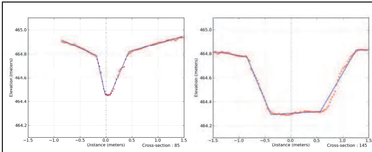
Fig. 12. Trapezoidal cross-sections fitted to measured data.
