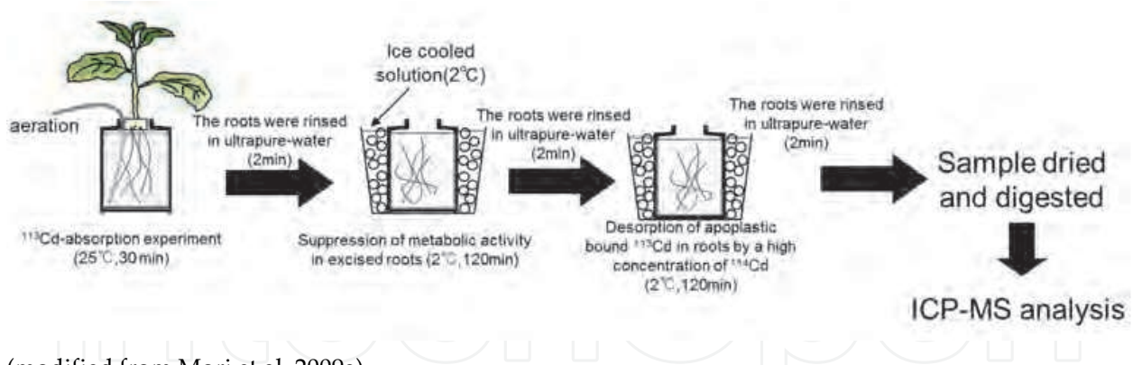
Fig. 1. Absorption experiment procedure for evaluating symplastic ^{113}\text{Cd} absorption in roots
