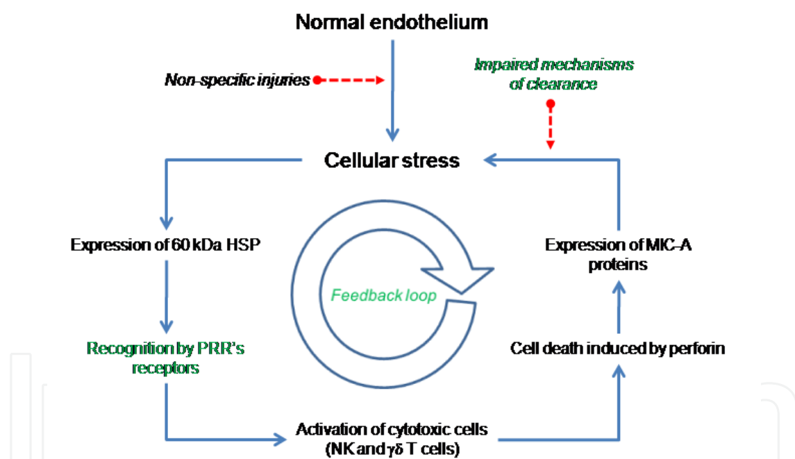
Fig. 1. A novel pathogenic model in Takayasu's arteritis. Non self-reactive phase. Unspecific damage factors induce stress in endothelial cells, which results in the expression of several stress-induced proteins, including 60 kDa heat shock protein (HSP). These stress-induced proteins are engaged by innate cytotoxic cells through pattern-recognition receptors (PPR's) and become activated, promoting apoptosis of vascular endothelial cells and enhancing the stressed cellular environment.
