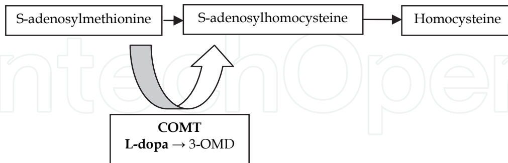
Fig. 2. COMT-mediated O-methylation of L-dopa, which results in formation of 3-methyldopa product, COMT- catecholamine-O-methyltransferase, 3-OMD- 3-O-methyldopa.
