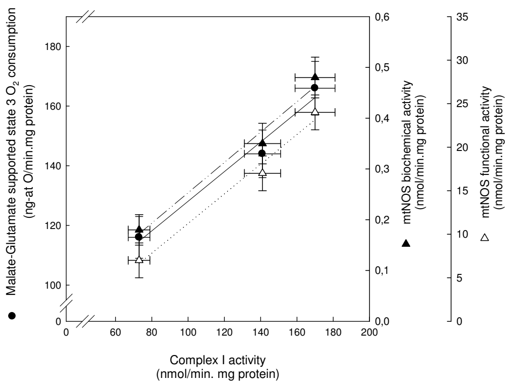
Fig. 1. Linear correlations between mitochondrial complex I activity and malate-glutamate supported state 3 respiration (●) ( r^2 = 0.97 ) and between mitochondrial complex I activity and mtNOS biochemical (▲) ( r^2 = 0.98 ) and functional activities (Δ) ( r^2 = 0.98 ).
