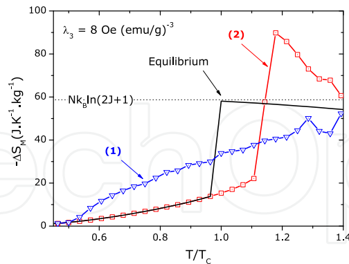
Fig. 18. -\Delta S_M(T) , obtained from the use of the Maxwell relation on equilibrium (black line) and metastable (colored lines) magnetization data from the Bean-Rodbell model with a magnetic field change of 1000 T.
