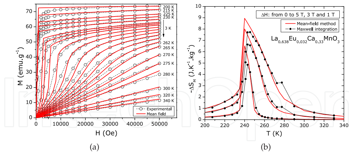
Fig. 14. Interpolating a) experimental M(H, T) data and b) magnetic entropy change results by mean-field simulations, of the first-order phase transition manganite \text{La}_{0.638}\text{Eu}_{0.032}\text{Ca}_{0.33}\text{MnO}_3 .
