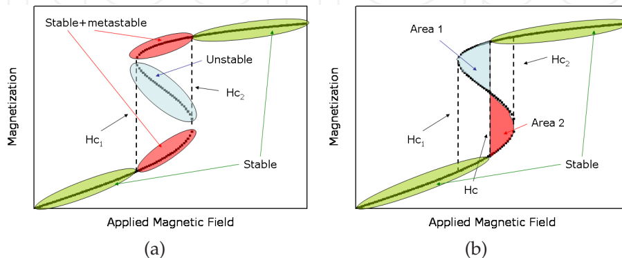
Fig. 2. a) The multiple solution branches from the roots of Eq. 22, for a first-order transition from the Bean-Rodbell model, and b) the Maxwell construction for determining the critical field H_c and the full equilibrium solution, for a first-order magnetic phase transition system.
