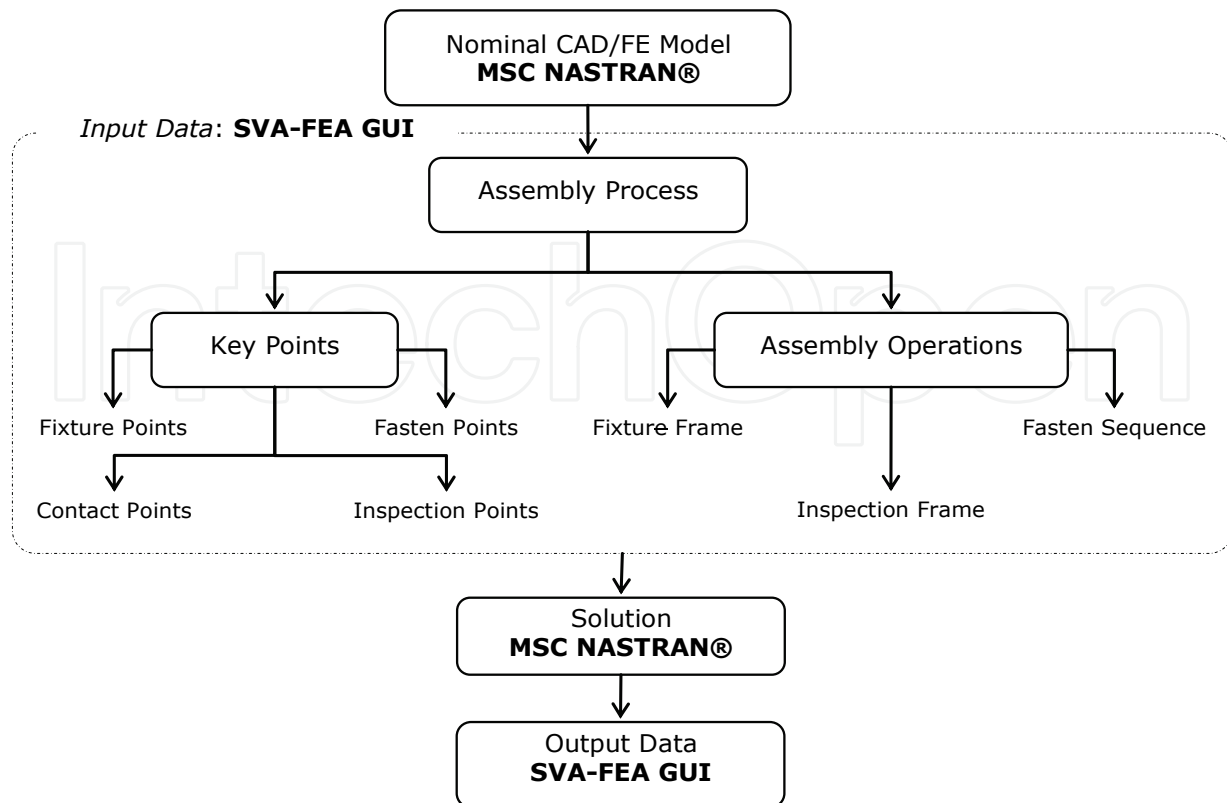
Fig. 2. SVA-FEA architecture (Franciosa, 2010a)
