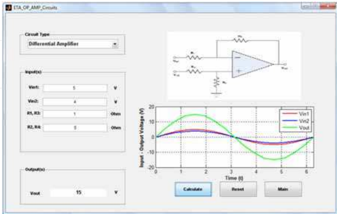
Fig. 18. Running the Differential Amplifier GUI
