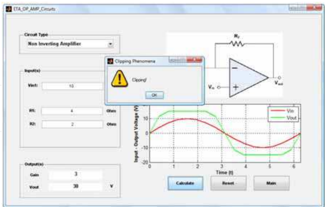
Fig. 19. Clipping Phenomena Warning Message
