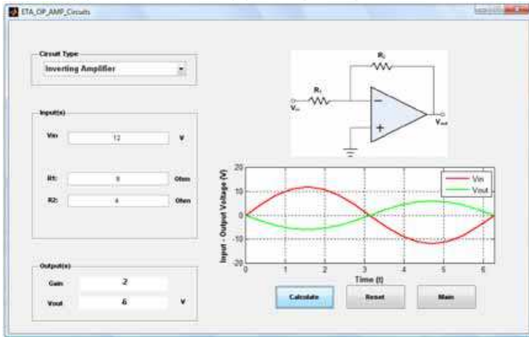
Fig. 14. Running the Inverting Amplifier GUI
