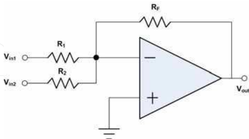
Fig. 5. The summing amplifier
