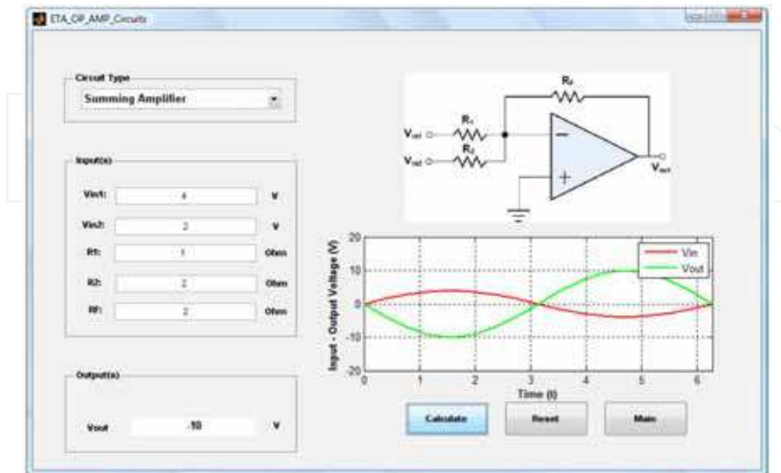
Fig. 16. Running the Summing Amplifier GUI
