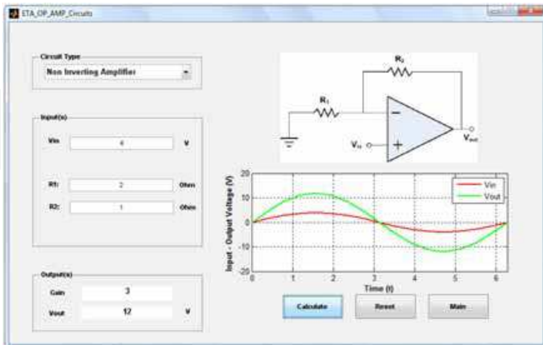
Fig. 15. Running the Non Inverting Amplifier GUI
