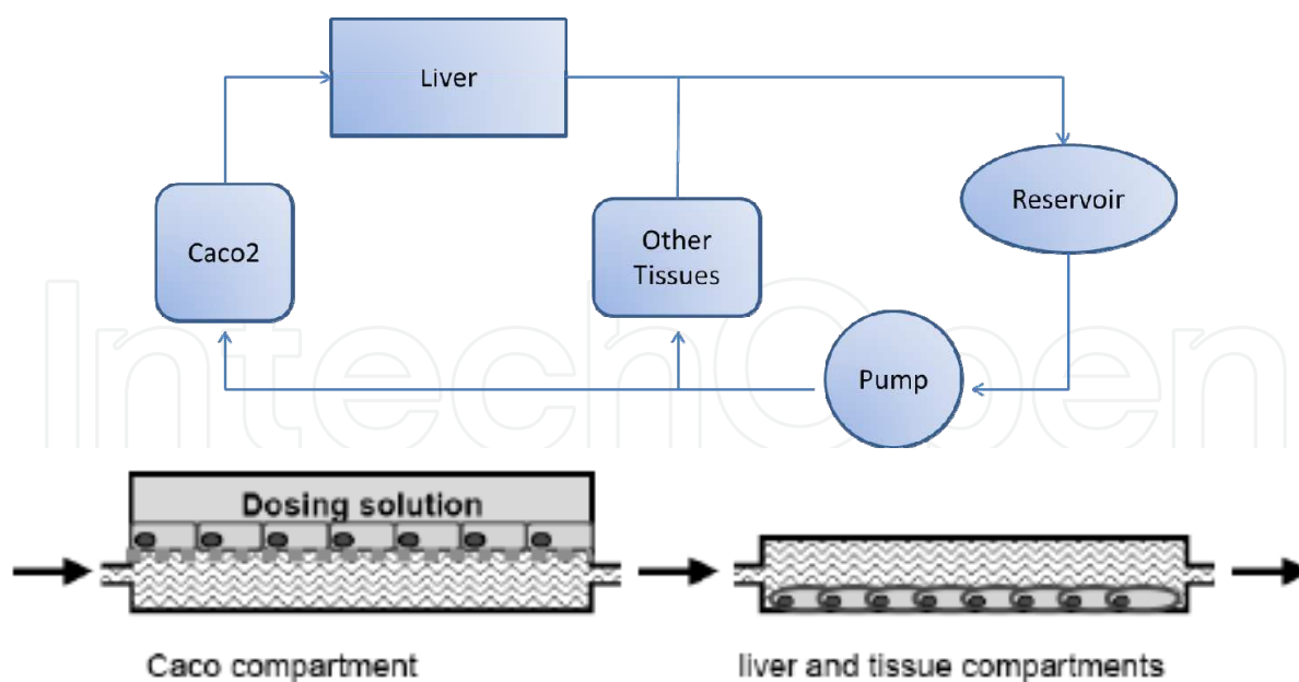
Fig. 6. Example of multi-compartmental MEMS model utilized to determine PBPK values for use in in silico simulations. The new chemical entity is dosed on one side of the Caco-2 cells, where it must be absorbed prior to reaching the microchannels. The absorbed drug then passes into the liver for metabolic clearance prior to being re-circulated and reaching the target tissue.
