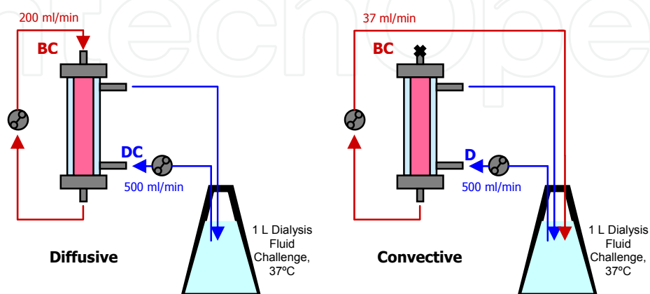
Fig. 1. Endotoxin challenge test setup, showing the blood loop and dialysis fluid loop flowrates for both diffusive and convective testing.
