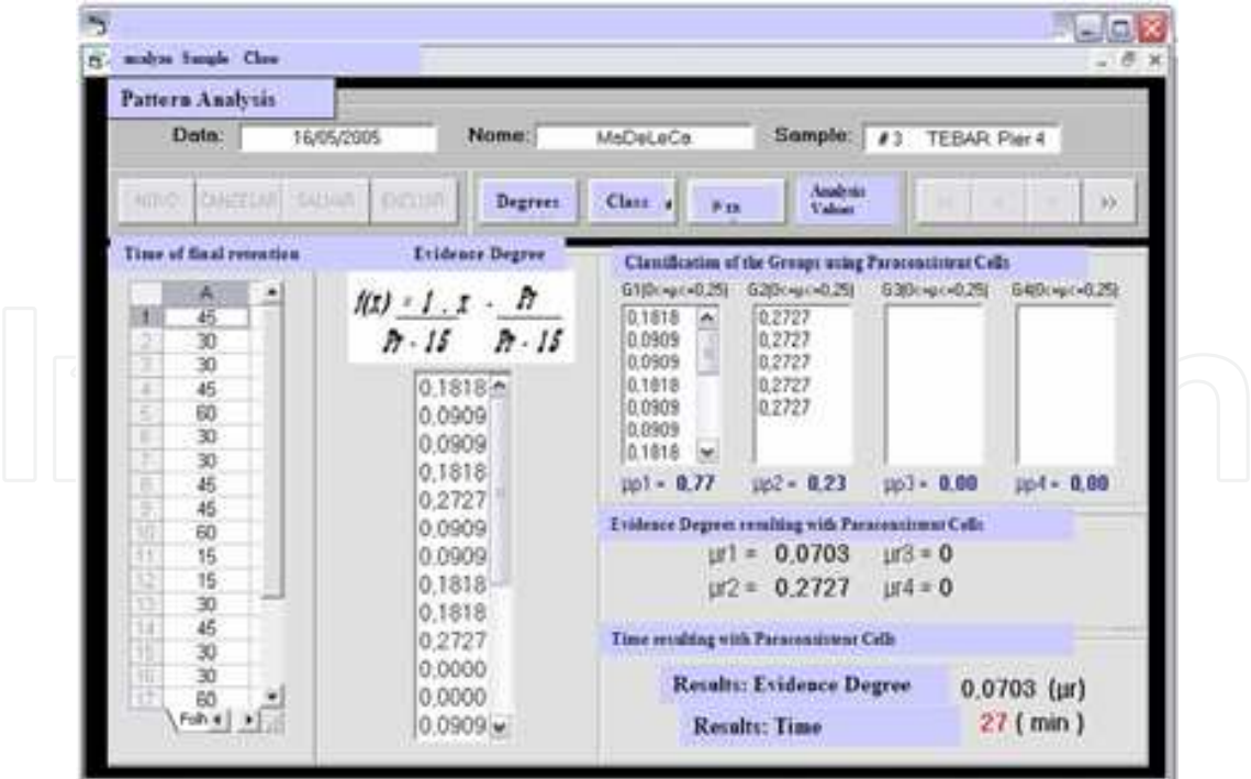
Fig. 15. Presentation of the result of analysis 1 of the pattern of reference done with the software elaborated with Paraconsistent Logic. Pr = 27min with the results in the form of Degrees of Evidence and classification of the tenor of sea pollution.
