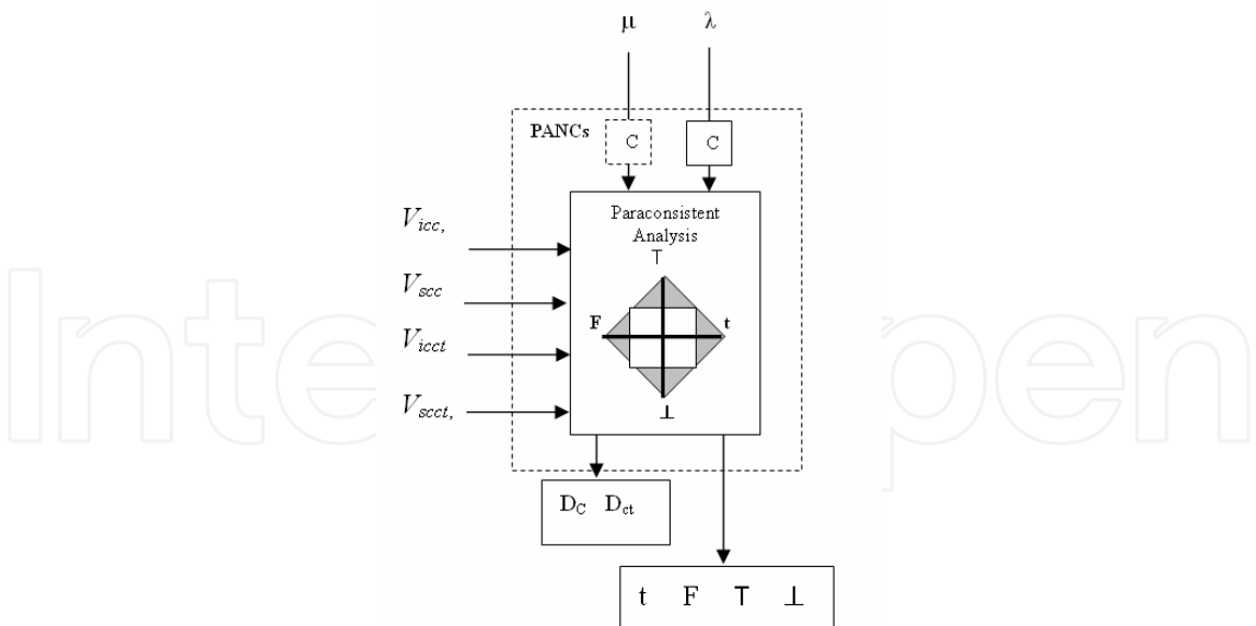
Fig. 3. The Basic Paraconsistent Artificial Neural Cell bPANC .
