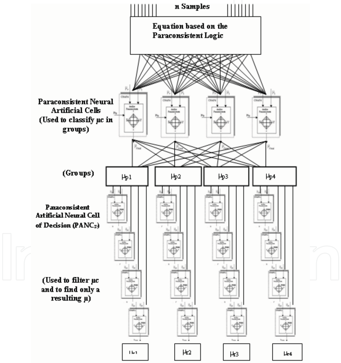
Fig. 10. The Paraconsistent network configuration. The next figure 11 shows the flow chart with the main steps of the treatment of signals.
