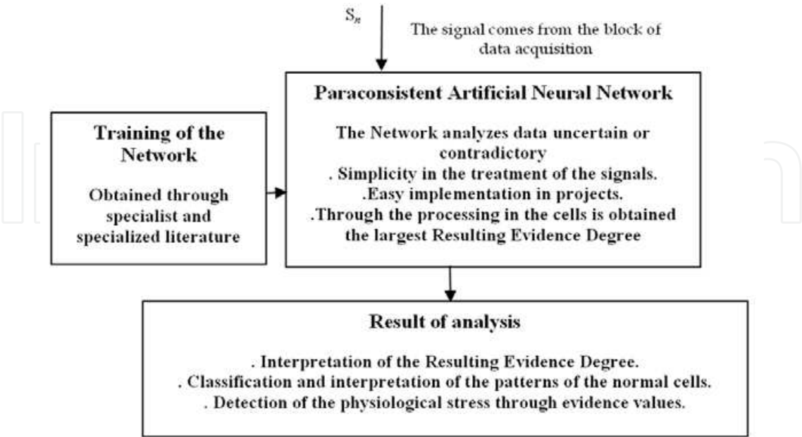
Fig. 8. Diagram in blocks of the Expert system with Paraconsistent Artificial Neural Networks applied to the method of obtaining the physiological stress cells.
