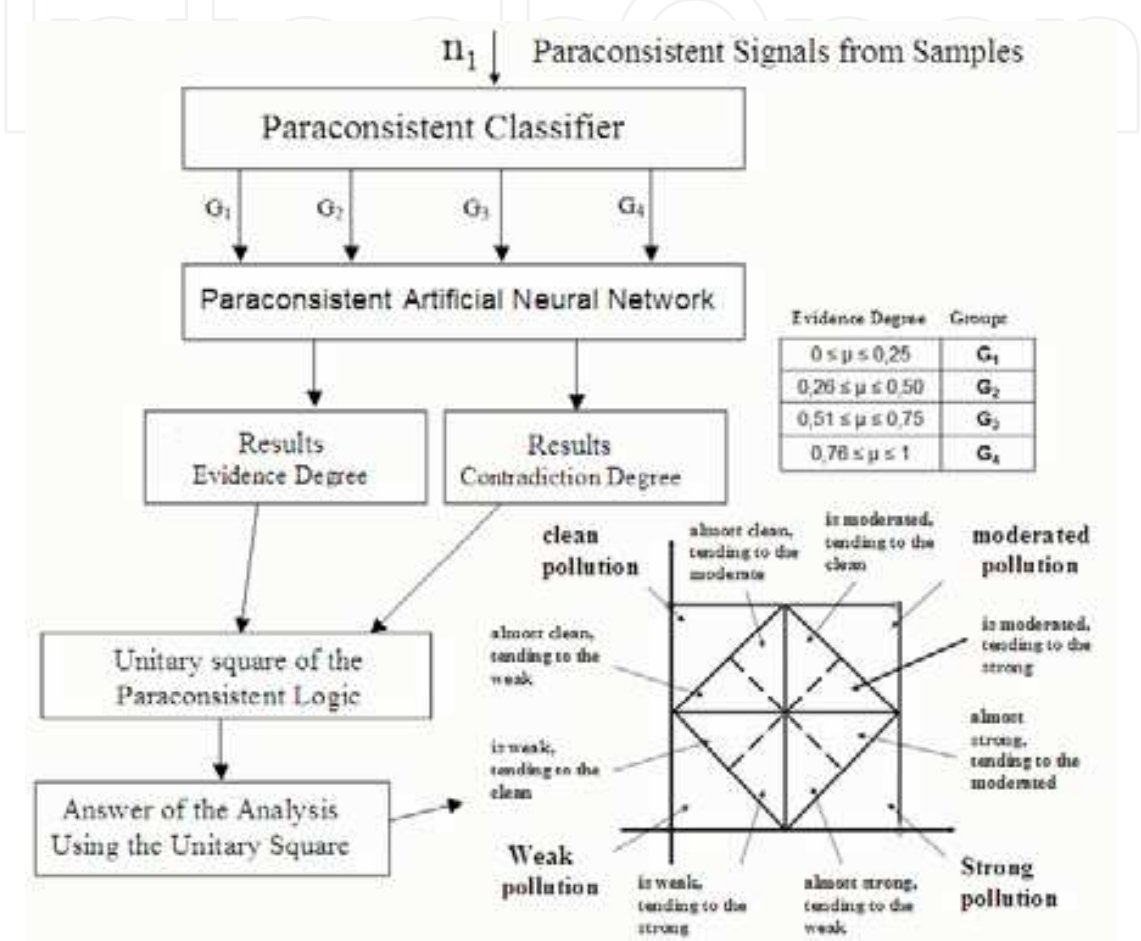
Fig. 13. Final Treatment and presentation of the results after classification and analysis of the Paraconsistent Signals.
